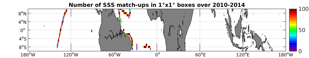
Figure 4: Number of SSS match-ups between TSG-GOSUD-Sailing-ship SSS and the SMOS-L3-CATDS-CECOS-LOCEAN-V2.1-9DAYS-25KM SSS product for the Equatorial Ocean 10N-10S Pi-MEP region over 1^\circ \times 1^\circ boxes and for the full satellite product period.
