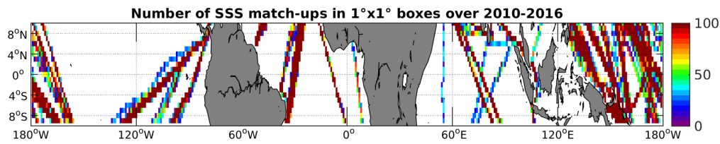
Figure 4: Number of SSS match-ups between TSG-LEGOS-DM SSS and the SMOS-L3-CATDS-CECOS-LOCEAN-V2-9DAYS-25KM SSS product for the Equatorial Ocean 10N-10S Pi-MEP region over 1^\circ \times 1^\circ boxes and for the full satellite product period.
