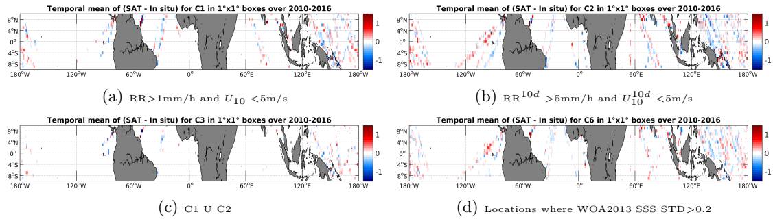
Figure 12: Temporal mean gridded over spatial boxes of size 1^\circ \times 1^\circ of \Delta SSS (SMOS-L3-CATDS-CECOS-LOCEAN-V2-9DAYS-25KM - TSG-LEGOS-DM) for 4 different subdatasets corresponding to: RR > 1\text{mm/h} and U_{10} < 5\text{m/s} (a), RR^{10d} > 5\text{mm/h} and U_{10}^{10d} < 5\text{m/s} (b), C1 U C2 (c), Locations where WOA2013 SSS STD > 0.2 (d).
