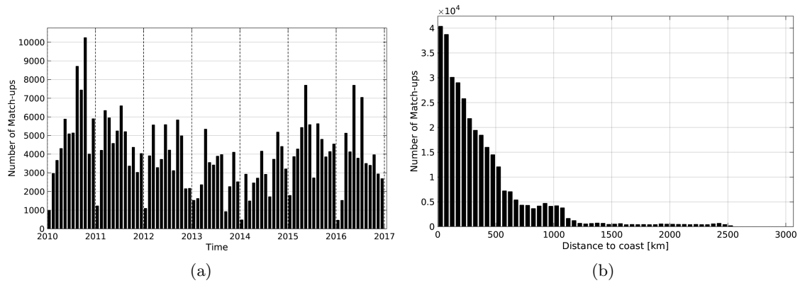
Figure 1: Number of match-ups between TSG-LEGOS-DM and SMOS-L3-CATDS-CECOS-LOCEAN-V2-9DAYS-25KM SSS as a function of time (a) and as function of the distance to coast (b) over the Equatorial Ocean 10N-10S Pi-MEP region and for the full satellite product period.
