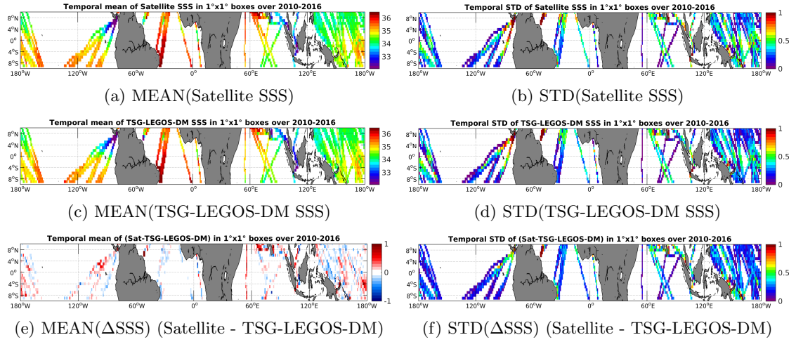
Figure 6: Temporal mean (left) and STD (right) of SSS from SMOS-L3-CATDS-CECOS-LOCEAN-V2-9DAYS-25KM (top), TSG-LEGOS-DM (middle), and of \Delta SSS (Satellite - TSG-LEGOS-DM). Only match-up pairs are used to generate these maps.
