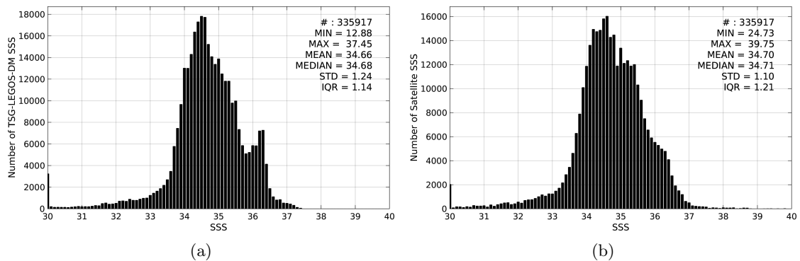
Figure 2: Histograms of SSS from TSG-LEGOS-DM (a) and SMOS-L3-CATDS-CECOS-LOCEAN-V2-9DAYS-25KM (b) considering all match-up pairs per bins of 0.1 over the Equatorial Ocean 10N-10S Pi-MEP region and for the full satellite product period.
