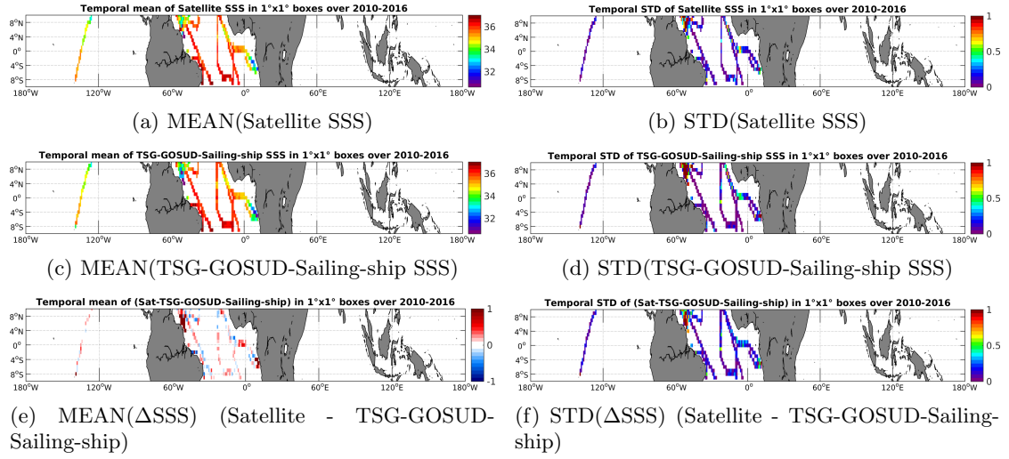
Figure 6: Temporal mean (left) and STD (right) of SSS from SMOS-L3-CATDS-CECOS-LOCEAN-V2-9DAYS-25KM (top), TSG-GOSUD-Sailing-ship (middle), and of \Delta SSS (Satellite - TSG-GOSUD-Sailing-ship). Only match-up pairs are used to generate these maps.
