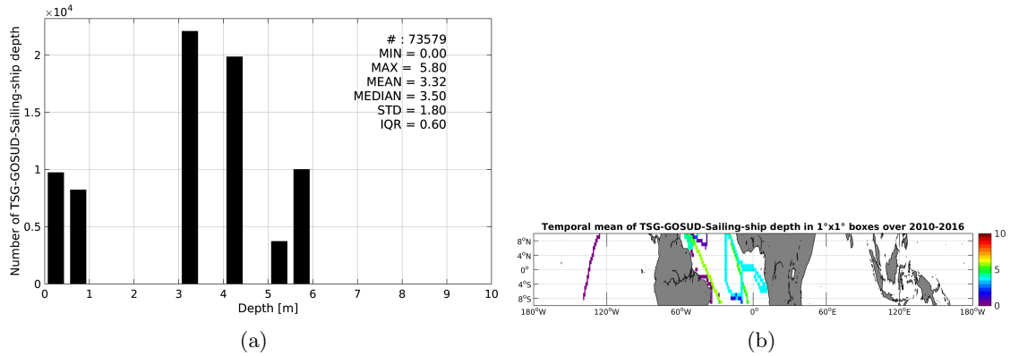
Figure 3: Histograms of the depth of the upper level SSS measurements from TSG-GOSUD-Sailing-ship in the Match-up DataBase for the Equatorial Ocean 10N-10S Pi-MEP region (a) and temporal mean spatial distribution of pressure of the in situ SSS data over 1^\circ \times 1^\circ boxes and for the full satellite product period (b).
