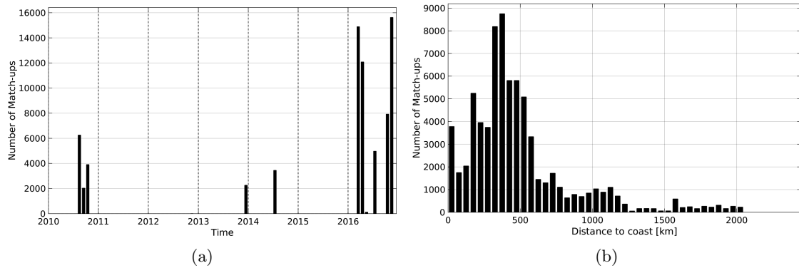
Figure 1: Number of match-ups between TSG-GOSUD-Sailing-ship and SMOS-L3-CATDS-CECOS-LOCEAN-V2-9DAYS-25KM SSS as a function of time (a) and as function of the distance to coast (b) over the Equatorial Ocean 10N-10S Pi-MEP region and for the full satellite product period.
