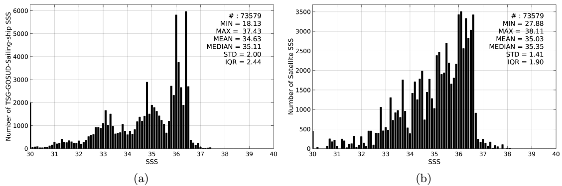
Figure 2: Histograms of SSS from TSG-GOSUD-Sailing-ship (a) and SMOS-L3-CATDS-CECOS-LOCEAN-V2-9DAYS-25KM (b) considering all match-up pairs per bins of 0.1 over the Equatorial Ocean 10N-10S Pi-MEP region and for the full satellite product period.
