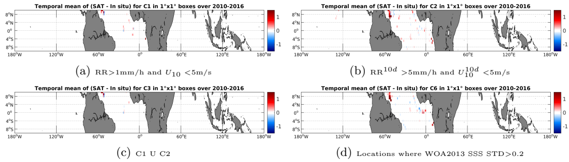
Figure 12: Temporal mean gridded over spatial boxes of size 1^\circ \times 1^\circ of \Delta SSS (SMOS-L3-CATDS-CECOS-LOCEAN-V2-9DAYS-25KM - TSG-GOSUD-Sailing-ship) for 4 different subdatasets corresponding to: RR > 1\text{mm/h} and U_{10} < 5\text{m/s} (a), RR^{10d} > 5\text{mm/h} and U_{10}^{10d} < 5\text{m/s} (b), C1 U C2 (c), Locations where WOA2013 SSS STD > 0.2 (d).
