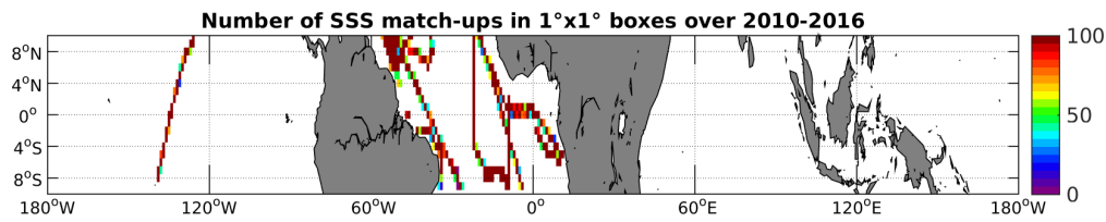
Figure 4: Number of SSS match-ups between TSG-GOSUD-Sailing-ship SSS and the SMOS-L3-CATDS-CECOS-LOCEAN-V2-9DAYS-25KM SSS product for the Equatorial Ocean 10N-10S Pi-MEP region over 1°x1° boxes and for the full satellite product period.
