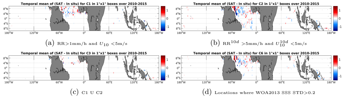
Figure 11: Temporal mean gridded over spatial boxes of size 1^\circ \times 1^\circ of \Delta SSS (SMOS-L3-CATDS-CECOS-LOCEAN-V2-9DAYS-25KM - Surface drifters) for 4 different subdatasets corresponding to: RR > 1\text{mm/h} and U_{10} < 5\text{m/s} (a), RR^{10d} > 5\text{mm/h} and U_{10}^{10d} < 5\text{m/s} (b), C1 U C2 (c), Locations where WOA2013 SSS STD > 0.2 (d).
