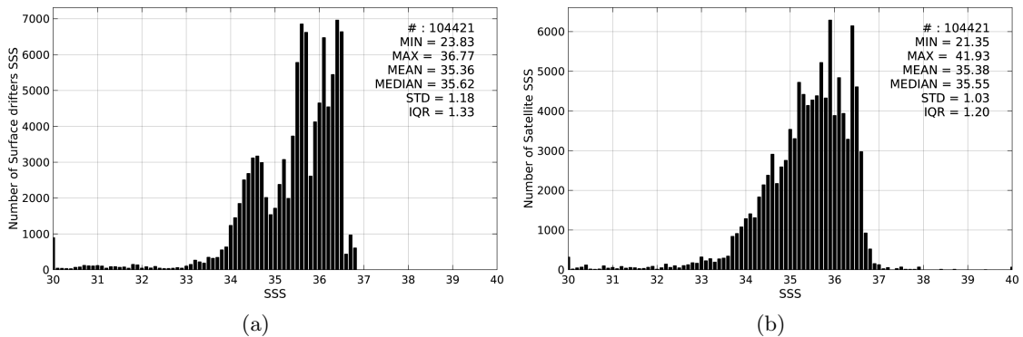
Figure 2: Histograms of SSS from Surface drifters (a) and SMOS-L3-CATDS-CECOS-LOCEAN-V2-9DAYS-25KM (b) considering all match-up pairs per bins of 0.1 over the Equatorial Ocean 10N-10S Pi-MEP region and for the full satellite product period.
