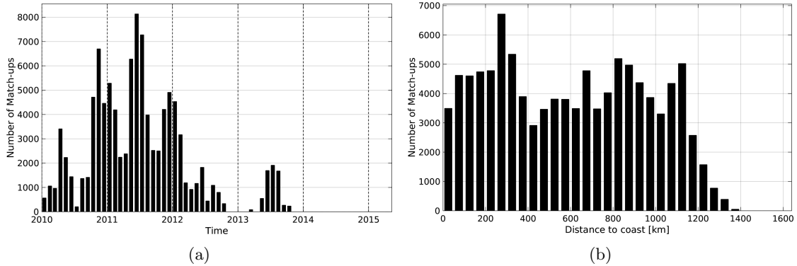
Figure 1: Number of match-ups between Surface drifters and SMOS-L3-CATDS-CECOS-LOCEAN-V2-9DAYS-25KM SSS as a function of time (a) and as function of the distance to coast (b) over the Equatorial Ocean 10N-10S Pi-MEP region and for the full satellite product period.
