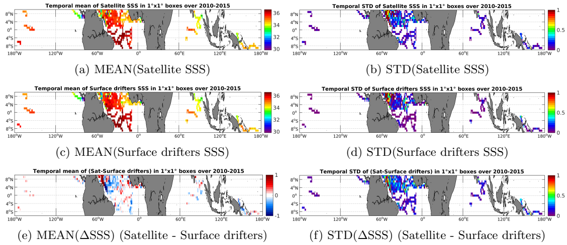
Figure 5: Temporal mean (left) and STD (right) of SSS from SMOS-L3-CATDS-CECOS-LOCEAN-V2-9DAYS-25KM (top), Surface drifters (middle), and of \Delta SSS (Satellite - Surface drifters). Only match-up pairs are used to generate these maps.
