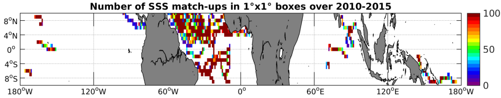
Figure 3: Number of SSS match-ups between Surface drifters SSS and the SMOS-L3-CATDS-CECOS-LOCEAN-V2-9DAYS-25KM SSS product for the Equatorial Ocean 10N-10S Pi-MEP region over 1^\circ \times 1^\circ boxes and for the full satellite product period.
