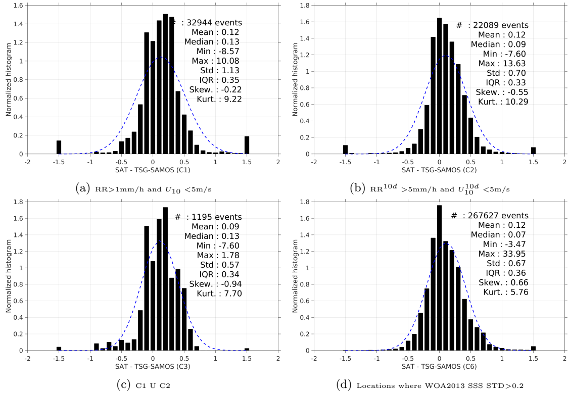
Figure 13: Normalized histogram of \Delta SSS (SMOS-L3-CATDS-CECOS-LOCEAN-V2-18DAYS-25KM - TSG-SAMOS) for 6 different subdatasets corresponding to: RR > 1\text{mm/h} and U_{10} < 5\text{m/s} (a), RR^{10d} > 5\text{mm/h} and U_{10}^{10d} < 5\text{m/s} (b), C1 U C2 (c), Locations where WOA2013 SSS STD > 0.2 (d).
