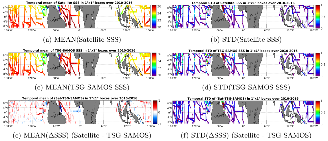
Figure 6: Temporal mean (left) and STD (right) of SSS from SMOS-L3-CATDS-CECOS-LOCEAN-V2-18DAYS-25KM (top), TSG-SAMOS (middle), and of \Delta SSS (Satellite - TSG-SAMOS). Only match-up pairs are used to generate these maps.
