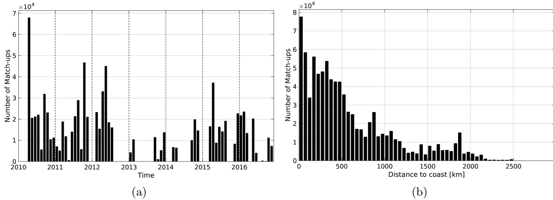
Figure 1: Number of match-ups between TSG-SAMOS and SMOS-L3-CATDS-CECOS-LOCEAN-V2-18DAYS-25KM SSS as a function of time (a) and as function of the distance to coast (b) over the Equatorial Ocean 10N-10S Pi-MEP region and for the full satellite product period.
