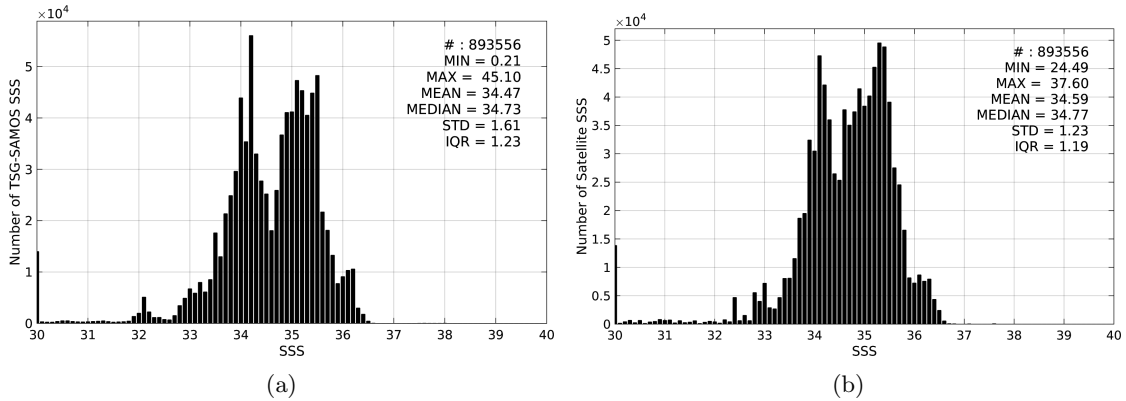
Figure 2: Histograms of SSS from TSG-SAMOS (a) and SMOS-L3-CATDS-CECOS-LOCEAN-V2-18DAYS-25KM (b) considering all match-up pairs per bins of 0.1 over the Equatorial Ocean 10N-10S Pi-MEP region and for the full satellite product period.
