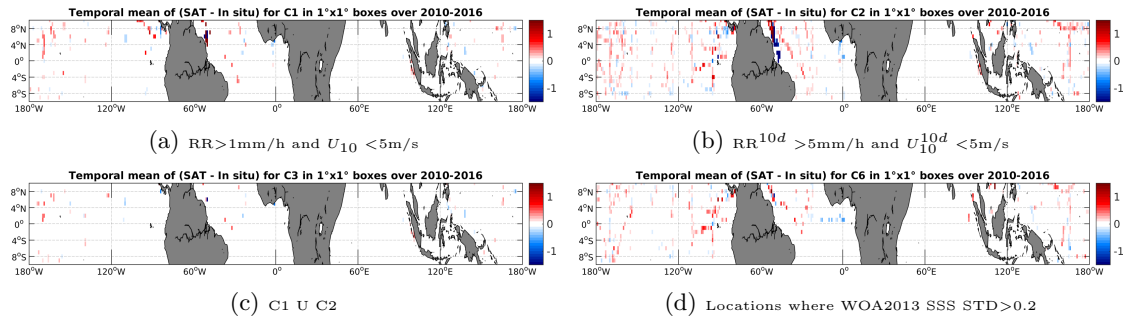
Figure 12: Temporal mean gridded over spatial boxes of size 1^\circ \times 1^\circ of \Delta SSS (SMOS-L3-CATDS-CECOS-LOCEAN-V2-18DAYS-25KM - TSG-SAMOS) for 4 different subdatasets corresponding to: RR > 1\text{mm/h} and U_{10} < 5\text{m/s} (a), RR^{10d} > 5\text{mm/h} and U_{10}^{10d} < 5\text{m/s} (b), C1 U C2 (c), Locations where WOA2013 SSS STD > 0.2 (d).
