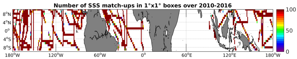
Figure 4: Number of SSS match-ups between TSG-SAMOS SSS and the SMOS-L3-CATDS-CECOS-LOCEAN-V2-18DAYS-25KM SSS product for the Equatorial Ocean 10N-10S Pi-MEP region over 1^\circ \times 1^\circ boxes and for the full satellite product period.
