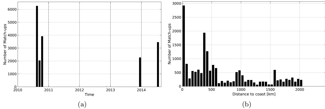
Figure 1: Number of match-ups between TSG-GOSUD-Sailing-ship and SMOS-L3-CATDS-CECOS-LOCEAN-V2-18DAYS-25KM SSS as a function of time (a) and as function of the distance to coast (b) over the Equatorial Ocean 10N-10S Pi-MEP region and for the full satellite product period.
