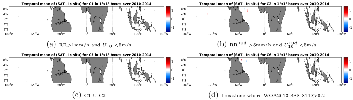
Figure 12: Temporal mean gridded over spatial boxes of size 1^\circ \times 1^\circ of \Delta SSS (SMOS-L3-CATDS-CECOS-LOCEAN-V2-18DAYS-25KM - TSG-GOSUD-Sailing-ship) for 4 different subdatasets corresponding to: RR > 1\text{mm/h} and U_{10} < 5\text{m/s} (a), RR^{10d} > 5\text{mm/h} and U_{10}^{10d} < 5\text{m/s} (b), C1 U C2 (c), Locations where WOA2013 SSS STD > 0.2 (d).
