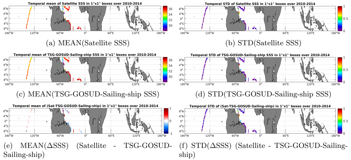
Figure 6: Temporal mean (left) and STD (right) of SSS from SMOS-L3-CATDS-CECOS-LOCEAN-V2-18DAYS-25KM (top), TSG-GOSUD-Sailing-ship (middle), and of \Delta SSS (Satellite - TSG-GOSUD-Sailing-ship). Only match-up pairs are used to generate these maps.
