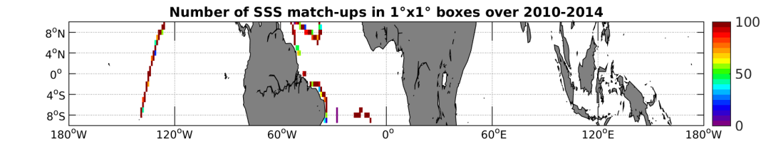
Figure 4: Number of SSS match-ups between TSG-GOSUD-Sailing-ship SSS and the SMOS-L3-CATDS-CECOS-LOCEAN-V2-18DAYS-25KM SSS product for the Equatorial Ocean 10N-10S Pi-MEP region over 1°x1° boxes and for the full satellite product period.
