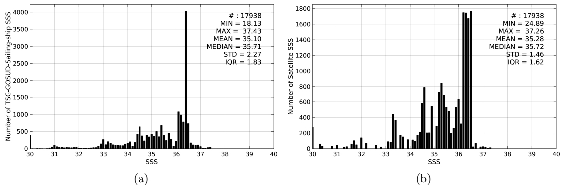
Figure 2: Histograms of SSS from TSG-GOSUD-Sailing-ship (a) and SMOS-L3-CATDS-CECOS-LOCEAN-V2-18DAYS-25KM (b) considering all match-up pairs per bins of 0.1 over the Equatorial Ocean 10N-10S Pi-MEP region and for the full satellite product period.
