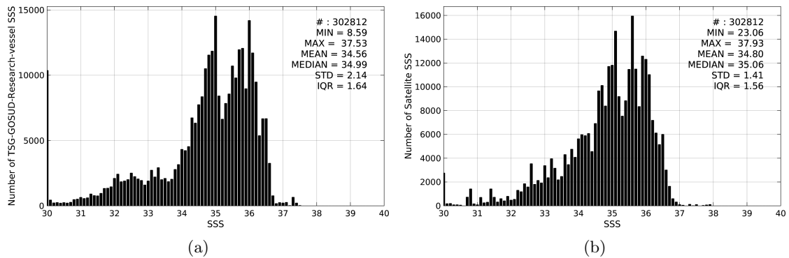
Figure 2: Histograms of SSS from TSG-GOSUD-Research-vessel (a) and SMOS-L3-CATDS-CECOS-LOCEAN-V2-18DAYS-25KM (b) considering all match-up pairs per bins of 0.1 over the Equatorial Ocean 10N-10S Pi-MEP region and for the full satellite product period.
