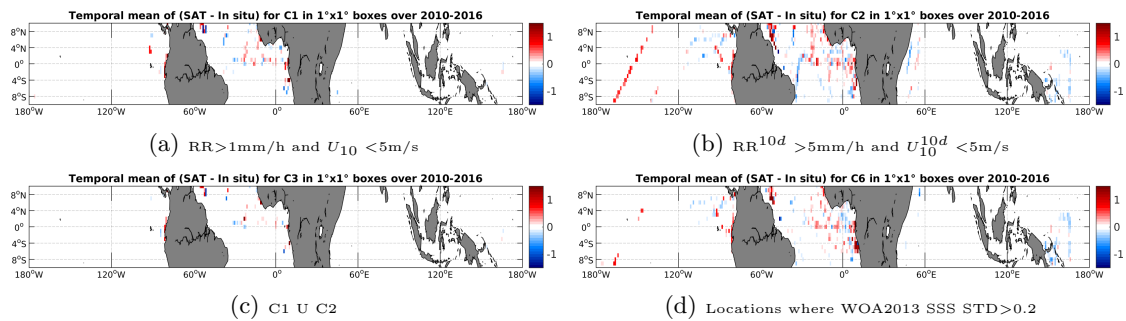
Figure 12: Temporal mean gridded over spatial boxes of size 1^\circ \times 1^\circ of \Delta SSS (SMOS-L3-CATDS-CECOS-LOCEAN-V2-18DAYS-25KM - TSG-GOSUD-Research-vessel) for 4 different subdatasets corresponding to: RR > 1\text{mm/h} and U_{10} < 5\text{m/s} (a), RR^{10d} > 5\text{mm/h} and U_{10}^{10d} < 5\text{m/s} (b), C1 U C2 (c),Locations where WOA2013 SSS STD > 0.2 (d).
