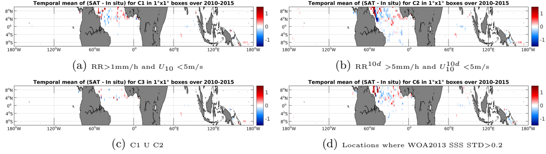
Figure 11: Temporal mean gridded over spatial boxes of size 1^\circ \times 1^\circ of \Delta SSS (SMOS-L3-CATDS-CECOS-LOCEAN-V2-18DAYS-25KM - Surface drifters) for 4 different subdatasets corresponding to: RR > 1 mm/h and U_{10} < 5 m/s (a), RR^{10d} > 5 mm/h and U_{10}^{10d} < 5 m/s (b), C1 U C2 (c), Locations where WOA2013 SSS STD > 0.2 (d).
