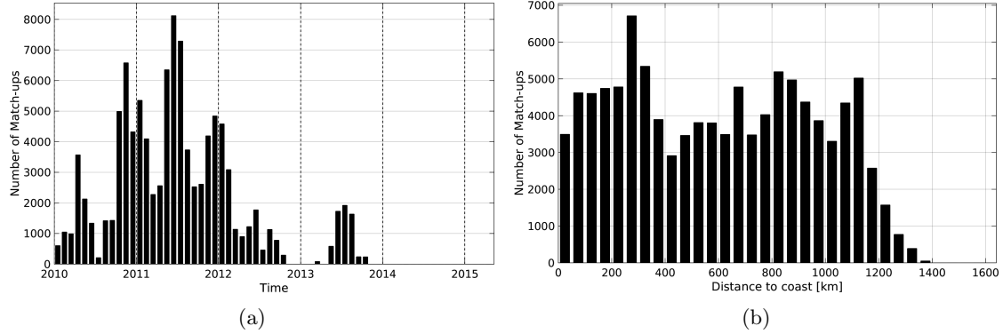
Figure 1: Number of match-ups between Surface drifters and SMOS-L3-CATDS-CECOS-LOCEAN-V2-18DAYS-25KM SSS as a function of time (a) and as function of the distance to coast (b) over the Equatorial Ocean 10N-10S Pi-MEP region and for the full satellite product period.
