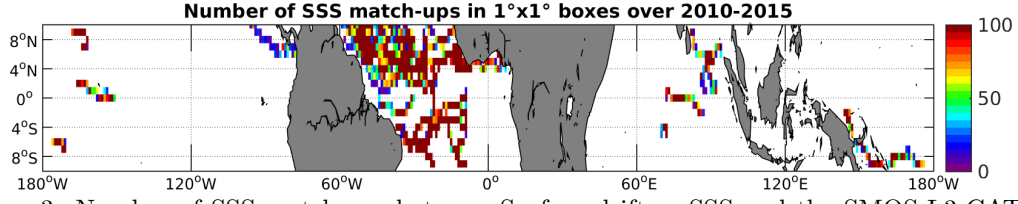
Figure 3: Number of SSS match-ups between Surface drifters SSS and the SMOS-L3-CATDS-CECOS-LOCEAN-V2-18DAYS-25KM SSS product for the Equatorial Ocean 10N-10S Pi-MEP region over 1°x1° boxes and for the full satellite product period.
