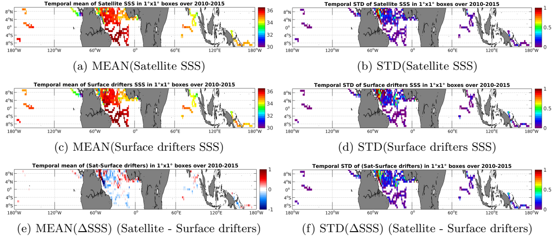
Figure 5: Temporal mean (left) and STD (right) of SSS from SMOS-L3-CATDS-CECOS-LOCEAN-V2-18DAYS-25KM (top), Surface drifters (middle), and of \Delta SSS (Satellite - Surface drifters). Only match-up pairs are used to generate these maps.
