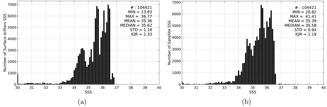
Figure 2: Histograms of SSS from Surface drifters (a) and SMOS-L3-CATDS-CECOS-LOCEAN-V2-18DAYS-25KM (b) considering all match-up pairs per bins of 0.1 over the Equatorial Ocean 10N-10S Pi-MEP region and for the full satellite product period.
