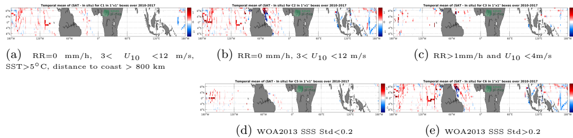
Figure 12: Temporal mean gridded over spatial boxes of size 1^{\circ}\times 1^{\circ} of \Delta\text{SSS} (SMOS SSS L3 v2 - Monthly - 0.25 Deg (CATDS-CECOS-IFREMER) - TSG (SAMOS)) for 5 different subdatasets corresponding to: RR=0 mm/h, 3 < U_{10} < 12 m/s, SST > 5^{\circ}\text{C} , distance to coast > 800 km (a), RR=0 mm/h, 3 < U_{10} < 12 m/s (b), RR > 1 mm/h and U_{10} < 4 m/s (c), WOA2013 SSS Std < 0.2 (d), WOA2013 SSS Std > 0.2 (e).
