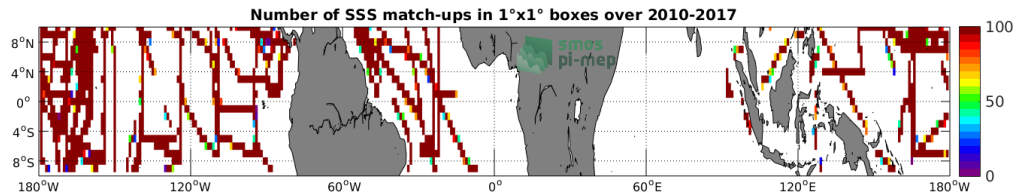
Figure 4: Number of SSS match-ups between TSG (SAMOS) SSS and the SMOS SSS L3 v2 - Monthly - 0.25 Deg (CATDS-CECOS-IFREMER) SSS product for the Equatorial Ocean 10N-10S Pi-MEP region over 1^\circ \times 1^\circ boxes and for the full satellite product period.
