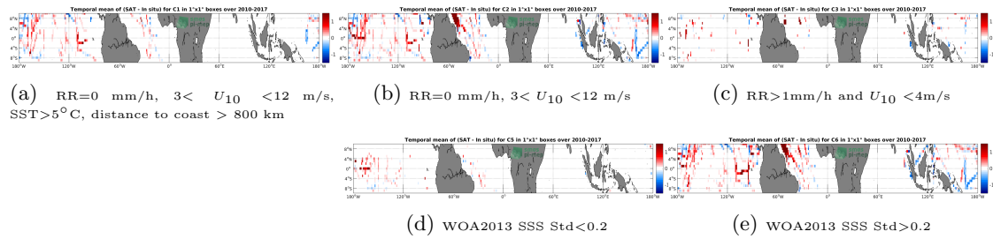
Figure 12: Temporal mean gridded over spatial boxes of size 1^\circ \times 1^\circ of \Delta SSS (SMOS-L3-CATDS-IFREMER-CECOS-V2-MONTHLY-0.25DEG - TSG-SAMOS) for 5 different subdatasets corresponding to:RR=0 mm/h, 3 < U_{10} < 12 m/s, SST >5^\circ C, distance to coast > 800 km (a), RR=0 mm/h, 3 < U_{10} < 12 m/s (b), RR >1 mm/h and U_{10} < 4 m/s (c), WOA2013 SSS Std <0.2 (d), WOA2013 SSS Std >0.2 (e).
