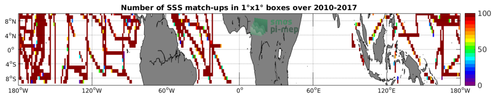
Figure 4: Number of SSS match-ups between TSG-SAMOS SSS and the SMOS-L3-CATDS-IFREMER-CECOS-V2-MONTHLY-0.25DEG SSS product for the Equatorial Ocean 10N-10S Pi-MEP region over 1^\circ \times 1^\circ boxes and for the full satellite product period.
