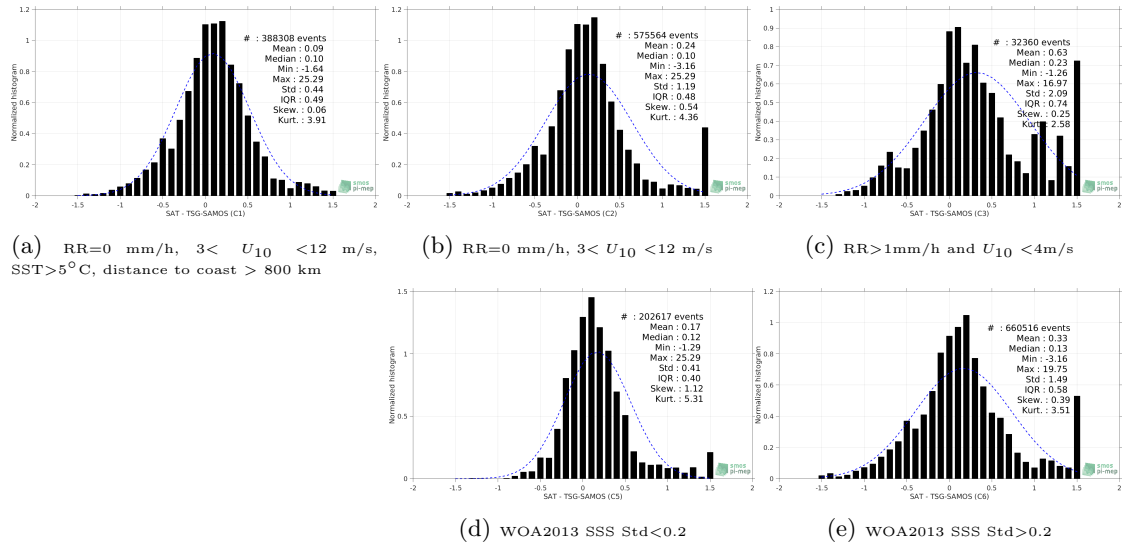
Figure 13: Normalized histogram of \Delta SSS (SMOS-L3-CATDS-IFREMER-CECOS-V2-MONTHLY-0.25DEG - TSG-SAMOS) for 5 different subdatasets corresponding to: RR=0 mm/h, 3 < U_{10} < 12 m/s, SST >5^\circ C, distance to coast > 800 km (a), RR=0 mm/h, 3 < U_{10} < 12 m/s (b), RR >1 mm/h and U_{10} < 4 m/s (c), WOA2013 SSS Std <0.2 (d), WOA2013 SSS Std >0.2 (e).
