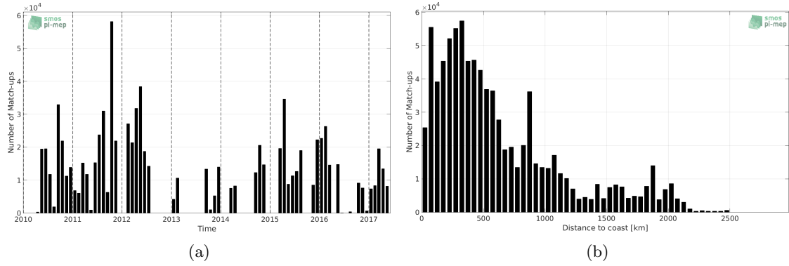
Figure 1: Number of match-ups between TSG-SAMOS and SMOS-L3-CATDS-IFREMER-CECOS-V2-MONTHLY-0.25DEG SSS as a function of time (a) and as function of the distance to coast (b) over the Equatorial Ocean 10N-10S Pi-MEP region and for the full satellite product period.
