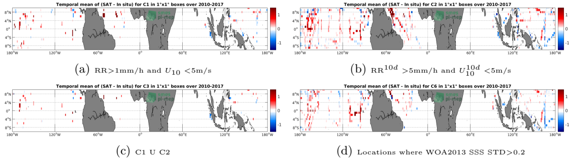
Figure 12: Temporal mean gridded over spatial boxes of size 1^\circ \times 1^\circ of \Delta SSS (SMOS-L3-CATDS-IFREMER-CECOS-V2-MONTHLY-0.25DEG - TSG-SAMOS) for 4 different subdatasets corresponding to: RR > 1\text{mm/h} and U_{10} < 5\text{m/s} (a), RR^{10d} > 5\text{mm/h} and U_{10}^{10d} < 5\text{m/s} (b), C1 U C2 (c), Locations where WOA2013 SSS STD > 0.2 (d).
