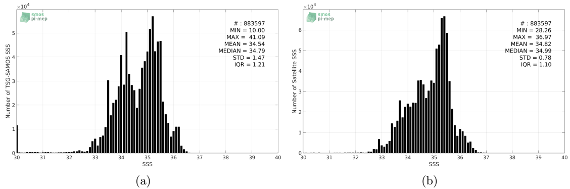
Figure 2: Histograms of SSS from TSG-SAMOS (a) and SMOS-L3-CATDS-IFREMER-CECOS-V2-MONTHLY-0.25DEG (b) considering all match-up pairs per bins of 0.1 over the Equatorial Ocean 10N-10S Pi-MEP region and for the full satellite product period.
