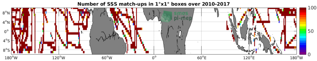
Figure 4: Number of SSS match-ups between TSG-SAMOS SSS and the SMOS-L3-CATDS-IFREMER-CECOS-V2-MONTHLY-0.25DEG SSS product for the Equatorial Ocean 10N-10S Pi-MEP region over 1°x1° boxes and for the full satellite product period.
