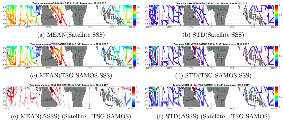
Figure 6: Temporal mean (left) and STD (right) of SSS from SMOS-L3-CATDS-IFREMER-CECOS-V2-MONTHLY-0.25DEG (top), TSG-SAMOS (middle), and of \Delta SSS (Satellite - TSG-SAMOS). Only match-up pairs are used to generate these maps.
