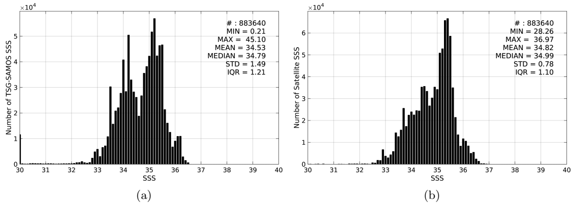
Figure 2: Histograms of SSS from TSG-SAMOS (a) and SMOS-L3-CATDS-IFREMER-CECOS-V2-MONTHLY-0.25DEG (b) considering all match-up pairs per bins of 0.1 over the Equatorial Ocean 10N-10S Pi-MEP region and for the full satellite product period.
