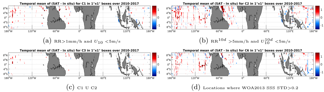
Figure 12: Temporal mean gridded over spatial boxes of size 1^\circ \times 1^\circ of \Delta SSS (SMOS-L3-CATDS-IFREMER-CECOS-V2-MONTHLY-0.25DEG - TSG-SAMOS) for 4 different subdatasets corresponding to: RR > 1\text{mm/h} and U_{10} < 5\text{m/s} (a), RR^{10d} > 5\text{mm/h} and U_{10}^{10d} < 5\text{m/s} (b), C1 U C2 (c), Locations where WOA2013 SSS STD > 0.2 (d).
