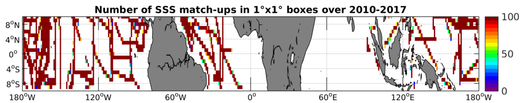
Figure 4: Number of SSS match-ups between TSG-SAMOS SSS and the SMOS-L3-CATDS-IFREMER-CECOS-V2-MONTHLY-0.25DEG SSS product for the Equatorial Ocean 10N-10S Pi-MEP region over 1^\circ \times 1^\circ boxes and for the full satellite product period.
