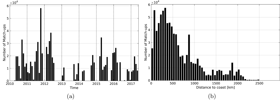
Figure 1: Number of match-ups between TSG-SAMOS and SMOS-L3-CATDS-IFREMER-CECOS-V2-MONTHLY-0.25DEG SSS as a function of time (a) and as function of the distance to coast (b) over the Equatorial Ocean 10N-10S Pi-MEP region and for the full satellite product period.
