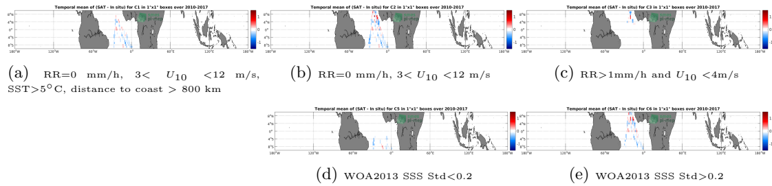
Figure 12: Temporal mean gridded over spatial boxes of size 1^{\circ}\times 1^{\circ} of \Delta\text{SSS} (SMOS SSS L3 v2 - Monthly - 0.25 Deg (CATDS-CECOS-IFREMER) - TSG (Polarstern)) for 5 different subdatasets corresponding to:RR=0 mm/h, 3 < U_{10} < 12 m/s, SST >5^{\circ}\text{C} , distance to coast > 800 km (a), RR=0 mm/h, 3 < U_{10} < 12 m/s (b), RR >1 mm/h and U_{10} < 4 m/s (c), WOA2013 SSS Std <0.2 (d), WOA2013 SSS Std >0.2 (e).
