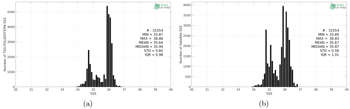
Figure 2: Histograms of SSS from TSG-POLARSTERN (a) and SMOS-L3-CATDS-IFREMER-CECOS-V2-MONTHLY-0.25DEG (b) considering all match-up pairs per bins of 0.1 over the Equatorial Ocean 10N-10S Pi-MEP region and for the full satellite product period.
