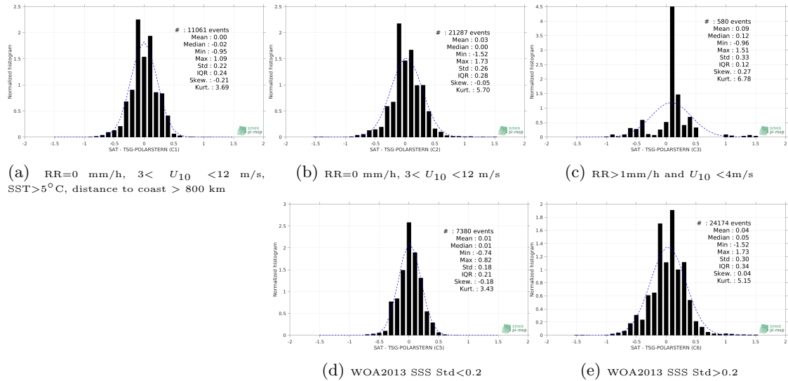
Figure 13: Normalized histogram of \Delta SSS (SMOS-L3-CATDS-IFREMER-CECOS-V2-MONTHLY-0.25DEG - TSG-POLARSTERN) for 5 different subdatasets corresponding to: RR=0 mm/h, 3 < U_{10} < 12 m/s, SST >5^\circ C, distance to coast > 800 km (a), RR=0 mm/h, 3 < U_{10} < 12 m/s (b), RR >1 mm/h and U_{10} < 4 m/s (c), WOA2013 SSS Std <0.2 (d), WOA2013 SSS Std >0.2 (e).
