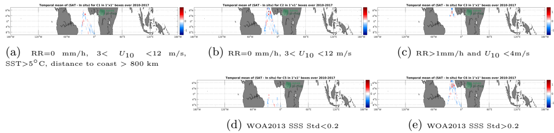
Figure 12: Temporal mean gridded over spatial boxes of size 1^\circ \times 1^\circ of \Delta SSS (SMOS-L3-CATDS-IFREMER-CECOS-V2-MONTHLY-0.25DEG - TSG-POLARSTERN) for 5 different subdatasets corresponding to:RR=0 mm/h, 3 < U_{10} < 12 m/s, SST >5^\circ C, distance to coast > 800 km (a), RR=0 mm/h, 3 < U_{10} < 12 m/s (b), RR >1 mm/h and U_{10} < 4 m/s (c), WOA2013 SSS Std <0.2 (d), WOA2013 SSS Std >0.2 (e).
