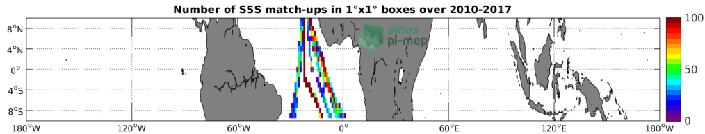
Figure 4: Number of SSS match-ups between TSG-POLARSTERN SSS and the SMOS-L3-CATDS-IFREMER-CECOS-V2-MONTHLY-0.25DEG SSS product for the Equatorial Ocean 10N-10S Pi-MEP region over 1^\circ \times 1^\circ boxes and for the full satellite product period.
