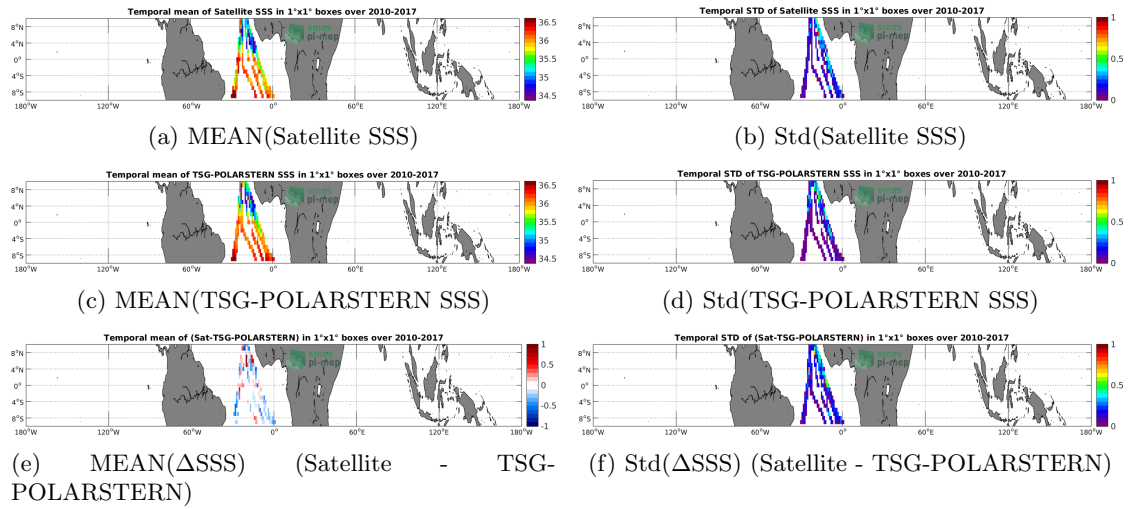
Figure 6: Temporal mean (left) and Std (right) of SSS from SMOS-L3-CATDS-IFREMER-CECOS-V2-MONTHLY-0.25DEG (top), TSG-POLARSTERN (middle), and of \Delta SSS (Satellite - TSG-POLARSTERN). Only match-up pairs are used to generate these maps.
