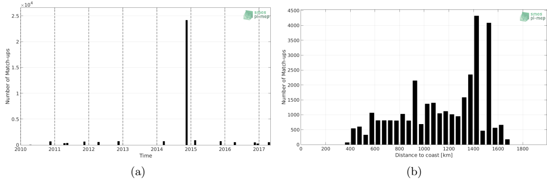
Figure 1: Number of match-ups between TSG-POLARSTERN and SMOS-L3-CATDS-IFREMER-CECOS-V2-MONTHLY-0.25DEG SSS as a function of time (a) and as function of the distance to coast (b) over the Equatorial Ocean 10N-10S Pi-MEP region and for the full satellite product period.
