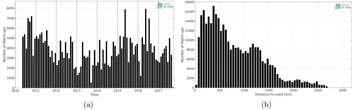
Figure 1: Number of match-ups between TSG-LEGOS-DM and SMOS L3 v2 - Monthly - 0.25 Deg (CATDS-CECOS-IFREMER) SSS as a function of time (a) and as function of the distance to coast (b) over the Equatorial Ocean 10N-10S Pi-MEP region and for the full satellite product period.
