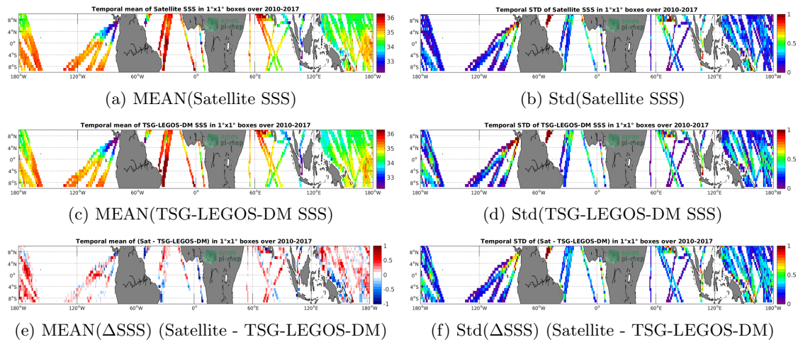
Figure 6: Temporal mean (left) and Std (right) of SSS from SMOS L3 v2 - Monthly - 0.25 Deg (CATDS-CECOS-IFREMER) (top), TSG-LEGOS-DM (middle), and of \Delta SSS (Satellite - TSG-LEGOS-DM). Only match-up pairs are used to generate these maps.
