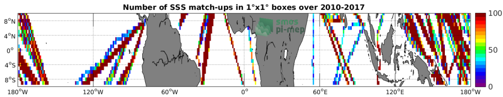
Figure 4: Number of SSS match-ups between TSG-LEGOS-DM SSS and the SMOS L3 v2 - Monthly - 0.25 Deg (CATDS-CECOS-IFREMER) SSS product for the Equatorial Ocean 10N-10S Pi-MEP region over 1°x1° boxes and for the full satellite product period.
