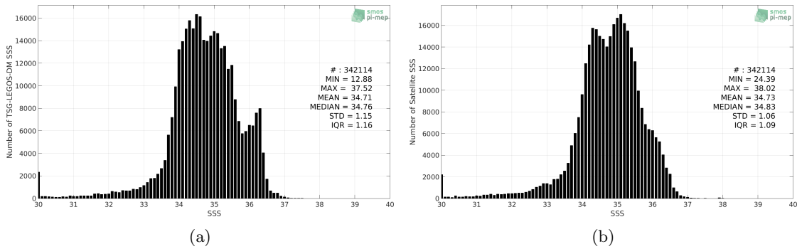
Figure 2: Histograms of SSS from TSG-LEGOS-DM (a) and SMOS L3 v2 - Monthly - 0.25 Deg (CATDS-CECOS-IFREMER) (b) considering all match-up pairs per bins of 0.1 over the Equatorial Ocean 10N-10S Pi-MEP region and for the full satellite product period.
