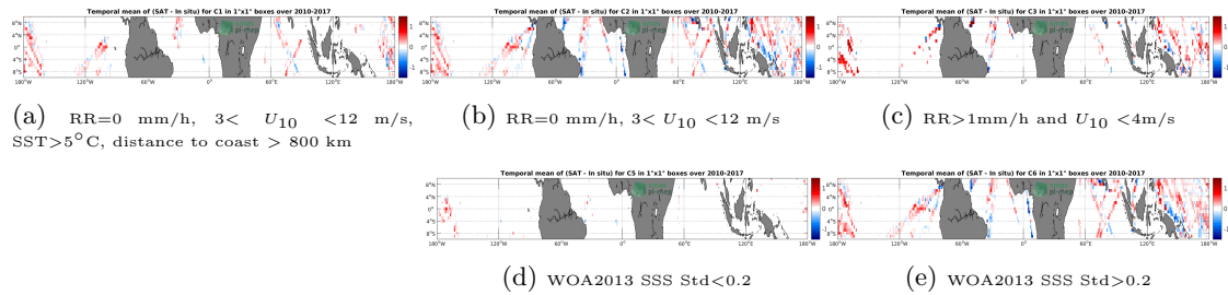
Figure 12: Temporal mean gridded over spatial boxes of size 1^{\circ}\times 1^{\circ} of \Delta\text{SSS} (SMOS L3 v2 - Monthly - 0.25 Deg (CATDS-CECOS-IFREMER) - TSG-LEGOS-DM) for 5 different subdatasets corresponding to:RR=0 mm/h, 3 < U_{10} < 12 m/s, SST >5^{\circ}\text{C} , distance to coast > 800 km (a), RR=0 mm/h, 3 < U_{10} < 12 m/s (b), RR >1 mm/h and U_{10} < 4 m/s (c), WOA2013 SSS Std <0.2 (d), WOA2013 SSS Std >0.2 (e).
