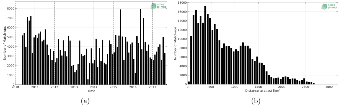
Figure 1: Number of match-ups between TSG-LEGOS-DM and SMOS-L3-CATDS-IFREMER-CECOS-V2-MONTHLY-0.25DEG SSS as a function of time (a) and as function of the distance to coast (b) over the Equatorial Ocean 10N-10S Pi-MEP region and for the full satellite product period.
