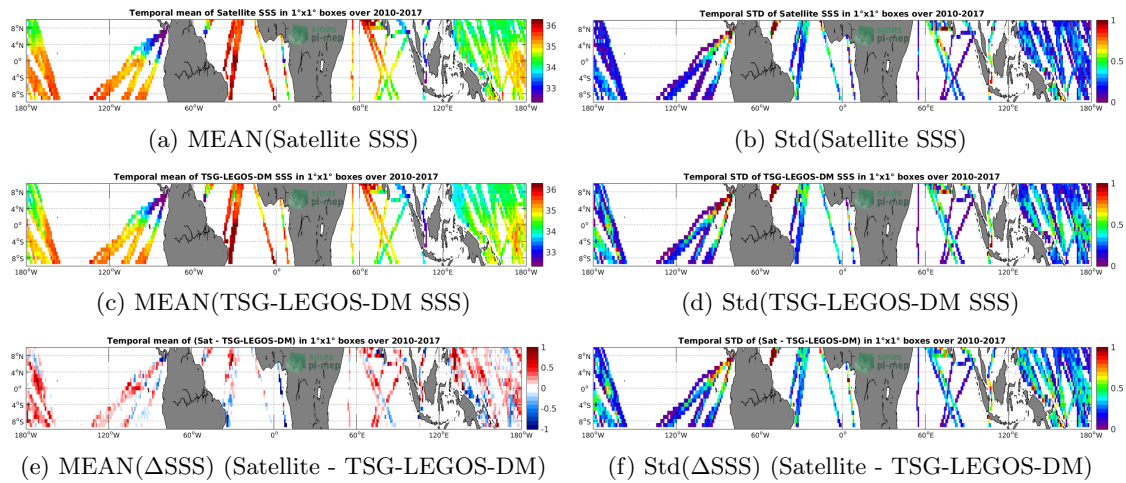
Figure 6: Temporal mean (left) and Std (right) of SSS from SMOS-L3-CATDS-IFREMER-CECOS-V2-MONTHLY-0.25DEG (top), TSG-LEGOS-DM (middle), and of \Delta SSS (Satellite - TSG-LEGOS-DM). Only match-up pairs are used to generate these maps.
