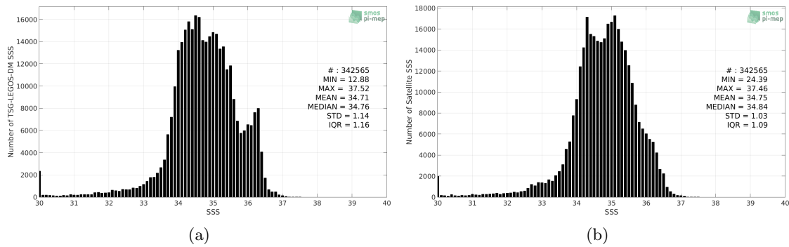
Figure 2: Histograms of SSS from TSG-LEGOS-DM (a) and SMOS-L3-CATDS-IFREMER-CECOS-V2-MONTHLY-0.25DEG (b) considering all match-up pairs per bins of 0.1 over the Equatorial Ocean 10N-10S Pi-MEP region and for the full satellite product period.
