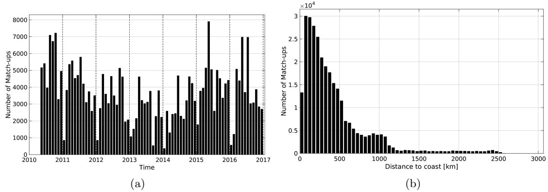
Figure 1: Number of match-ups between TSG-LEGOS-DM and SMOS-L3-CATDS-IFREMER-CECOS-V2-MONTHLY-0.25DEG SSS as a function of time (a) and as function of the distance to coast (b) over the Equatorial Ocean 10N-10S Pi-MEP region and for the full satellite product period.
