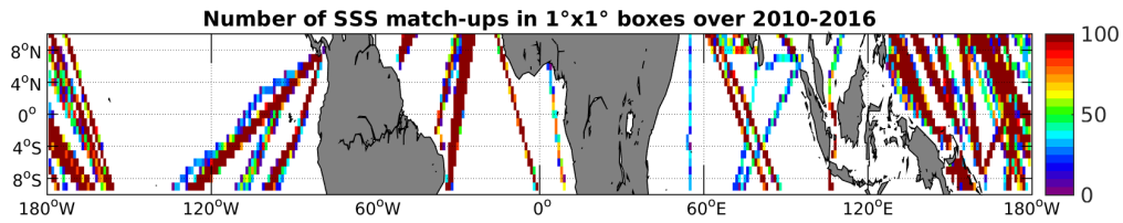
Figure 4: Number of SSS match-ups between TSG-LEGOS-DM SSS and the SMOS-L3-CATDS-IFREMER-CECOS-V2-MONTHLY-0.25DEG SSS product for the Equatorial Ocean 10N-10S Pi-MEP region over 1^\circ \times 1^\circ boxes and for the full satellite product period.
