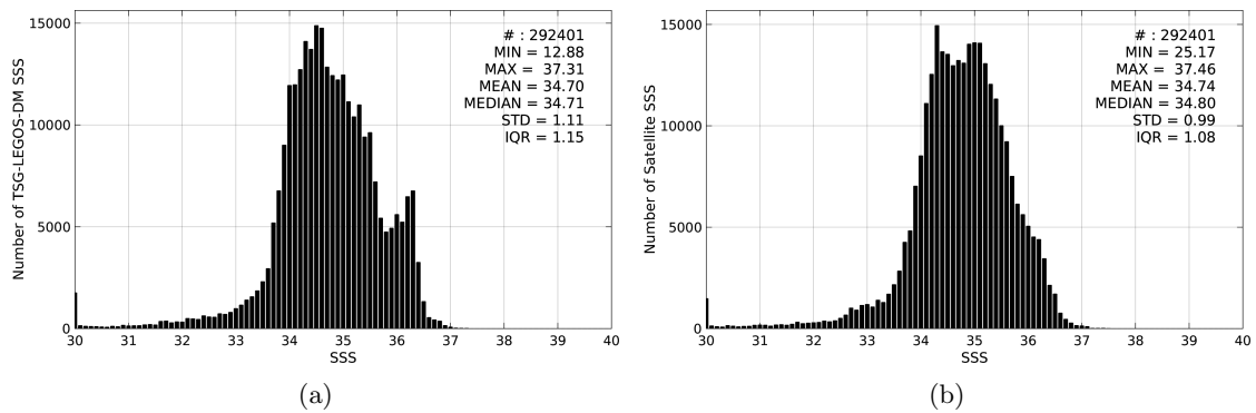
Figure 2: Histograms of SSS from TSG-LEGOS-DM (a) and SMOS-L3-CATDS-IFREMER-CECOS-V2-MONTHLY-0.25DEG (b) considering all match-up pairs per bins of 0.1 over the Equatorial Ocean 10N-10S Pi-MEP region and for the full satellite product period.
