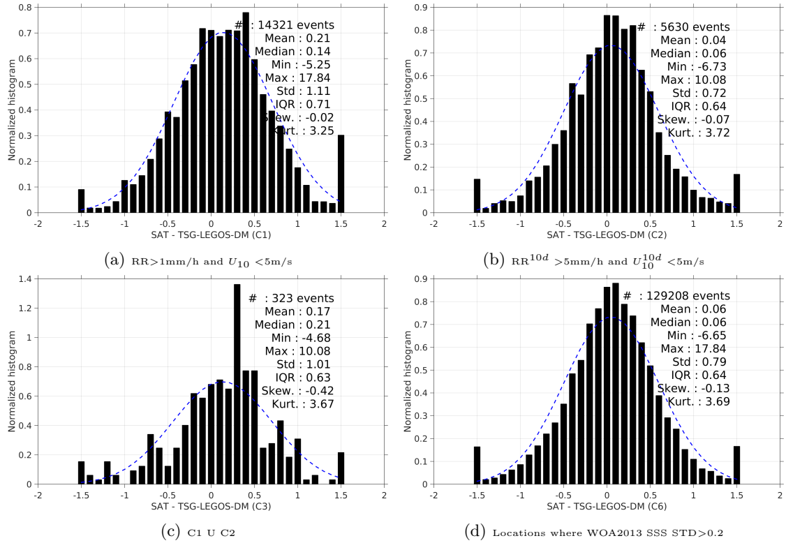
Figure 13: Normalized histogram of \Delta\text{SSS} (SMOS-L3-CATDS-IFREMER-CECOS-V2-MONTHLY-0.25DEG - TSG-LEGOS-DM) for 6 different subdatasets corresponding to: RR > 1mm/h and U_{10} < 5\text{m/s} (a), RR^{10d} > 5\text{mm/h} and U_{10}^{10d} < 5\text{m/s} (b), C1 U C2 (c), Locations where WOA2013 SSS STD > 0.2 (d).
