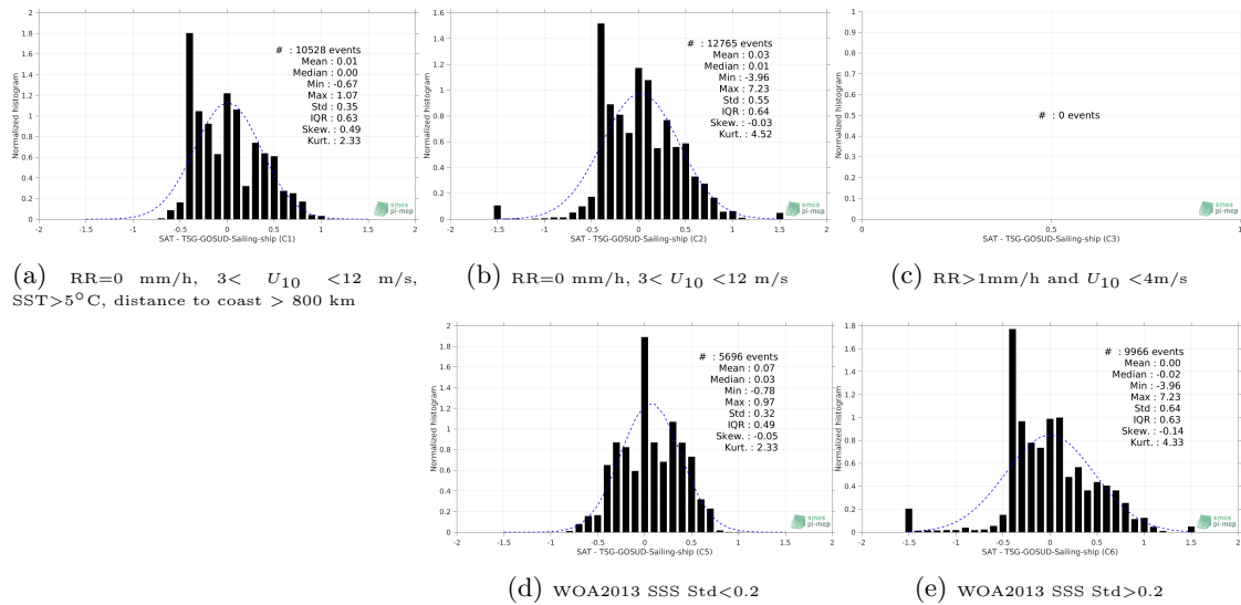
Figure 13: Normalized histogram of \Delta SSS (SMOS-L3-CATDS-IFREMER-CECOS-V2-MONTHLY-0.25DEG - TSG-GOSUD-Sailing-ship) for 5 different sub-datasets corresponding to: RR=0 mm/h, 3 < U_{10} < 12 m/s, SST >5^\circ C, distance to coast > 800 km (a), RR=0 mm/h, 3 < U_{10} < 12 m/s (b), RR >1 mm/h and U_{10} < 4 m/s (c), WOA2013 SSS Std <0.2 (d), WOA2013 SSS Std >0.2 (e).
