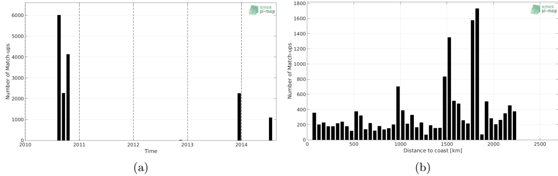
Figure 1: Number of match-ups between TSG-GOSUD-Sailing-ship and SMOS-L3-CATDS-IFREMER-CECOS-V2-MONTHLY-0.25DEG SSS as a function of time (a) and as function of the distance to coast (b) over the Equatorial Ocean 10N-10S Pi-MEP region and for the full satellite product period.
