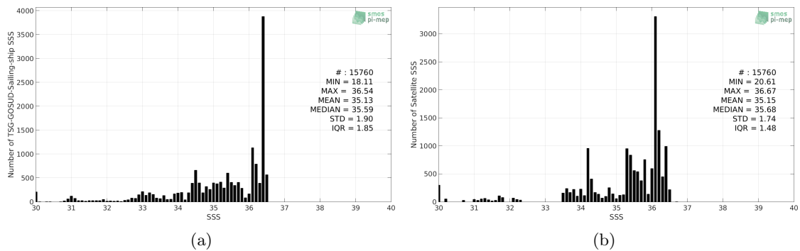
Figure 2: Histograms of SSS from TSG-GOSUD-Sailing-ship (a) and SMOS-L3-CATDS-IFREMER-CECOS-V2-MONTHLY-0.25DEG (b) considering all match-up pairs per bins of 0.1 over the Equatorial Ocean 10N-10S Pi-MEP region and for the full satellite product period.
