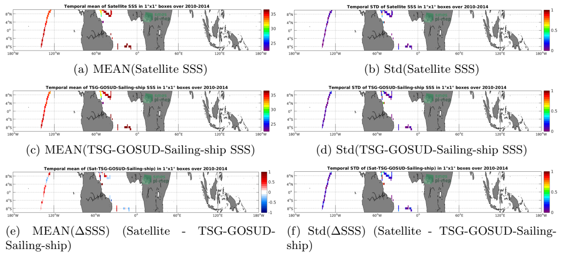
Figure 6: Temporal mean (left) and Std (right) of SSS from SMOS-L3-CATDS-IFREMER-CECOS-V2-MONTHLY-0.25DEG (top), TSG-GOSUD-Sailing-ship (middle), and of \Delta SSS (Satellite - TSG-GOSUD-Sailing-ship). Only match-up pairs are used to generate these maps.
