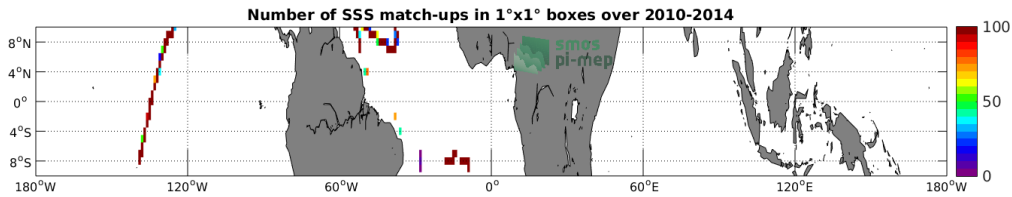
Figure 4: Number of SSS match-ups between TSG-GOSUD-Sailing-ship SSS and the SMOS-L3-CATDS-IFREMER-CECOS-V2-MONTHLY-0.25DEG SSS product for the Equatorial Ocean 10N-10S Pi-MEP region over 1^\circ \times 1^\circ boxes and for the full satellite product period.
