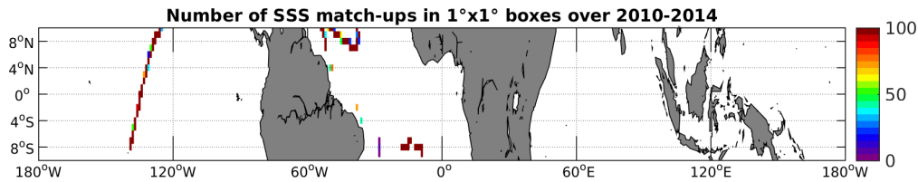
Figure 4: Number of SSS match-ups between TSG-GOSUD-Sailing-ship SSS and the SMOS-L3-CATDS-IFREMER-CECOS-V2-MONTHLY-0.25DEG SSS product for the Equatorial Ocean 10N-10S Pi-MEP region over 1^\circ \times 1^\circ boxes and for the full satellite product period.
