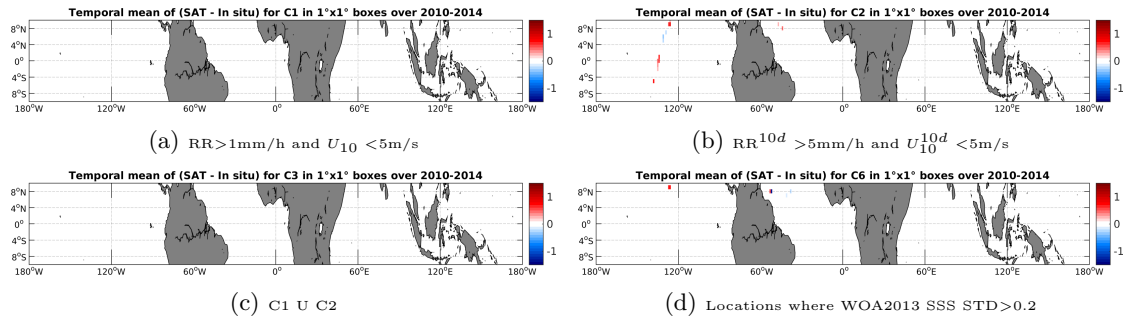
Figure 12: Temporal mean gridded over spatial boxes of size 1^\circ \times 1^\circ of \Delta SSS (SMOS-L3-CATDS-IFREMER-CECOS-V2-MONTHLY-0.25DEG - TSG-GOSUD-Sailing-ship) for 4 different sub-datasets corresponding to: RR > 1\text{mm/h} and U_{10} < 5\text{m/s} (a), RR^{10d} > 5\text{mm/h} and U_{10}^{10d} < 5\text{m/s} (b), C1 U C2 (c), Locations where WOA2013 SSS STD > 0.2 (d).
