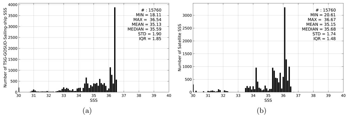
Figure 2: Histograms of SSS from TSG-GOSUD-Sailing-ship (a) and SMOS-L3-CATDS-IFREMER-CECOS-V2-MONTHLY-0.25DEG (b) considering all match-up pairs per bins of 0.1 over the Equatorial Ocean 10N-10S Pi-MEP region and for the full satellite product period.
