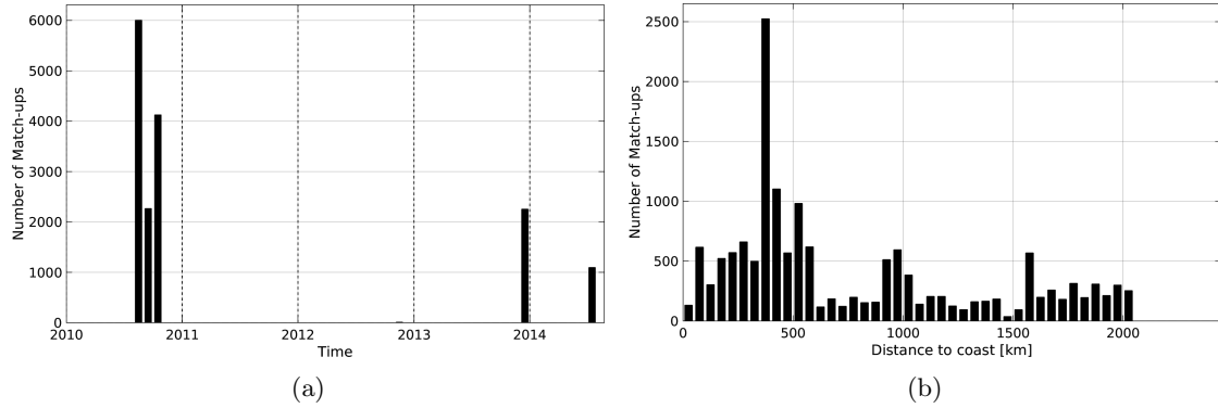
Figure 1: Number of match-ups between TSG-GOSUD-Sailing-ship and SMOS-L3-CATDS-IFREMER-CECOS-V2-MONTHLY-0.25DEG SSS as a function of time (a) and as function of the distance to coast (b) over the Equatorial Ocean 10N-10S Pi-MEP region and for the full satellite product period.
