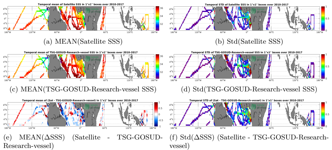
Figure 6: Temporal mean (left) and Std (right) of SSS from SMOS L3 v2 - Monthly - 0.25 Deg (CATDS-CECOS-IFREMER) (top), TSG-GOSUD-Research-vessel (middle), and of \Delta SSS (Satellite - TSG-GOSUD-Research-vessel). Only match-up pairs are used to generate these maps.
