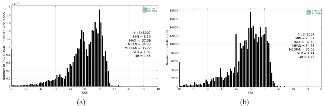
Figure 2: Histograms of SSS from TSG-GOSUD-Research-vessel (a) and SMOS L3 v2 - Monthly - 0.25 Deg (CATDS-CECOS-IFREMER) (b) considering all match-up pairs per bins of 0.1 over the Equatorial Ocean 10N-10S Pi-MEP region and for the full satellite product period.
