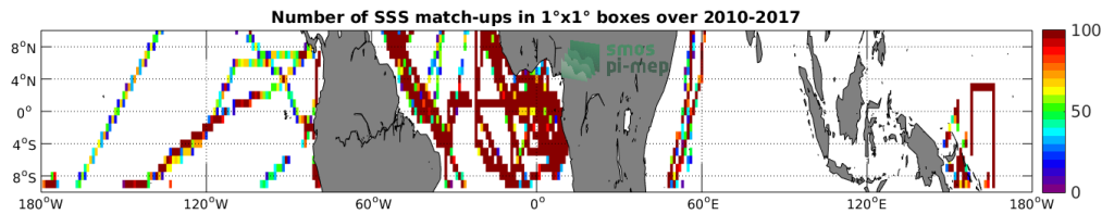
Figure 4: Number of SSS match-ups between TSG-GOSUD-Research-vessel SSS and the SMOS L3 v2 - Monthly - 0.25 Deg (CATDS-CECOS-IFREMER) SSS product for the Equatorial Ocean 10N-10S Pi-MEP region over 1^\circ \times 1^\circ boxes and for the full satellite product period.
