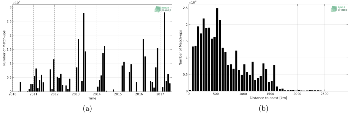
Figure 1: Number of match-ups between TSG-GOSUD-Research-vessel and SMOS-L3-CATDS-IFREMER-CECOS-V2-MONTHLY-0.25DEG SSS as a function of time (a) and as function of the distance to coast (b) over the Equatorial Ocean 10N-10S Pi-MEP region and for the full satellite product period.
