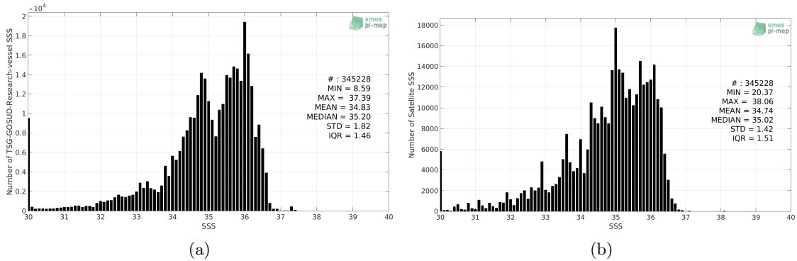
Figure 2: Histograms of SSS from TSG-GOSUD-Research-vessel (a) and SMOS-L3-CATDS-IFREMER-CECOS-V2-MONTHLY-0.25DEG (b) considering all match-up pairs per bins of 0.1 over the Equatorial Ocean 10N-10S Pi-MEP region and for the full satellite product period.
