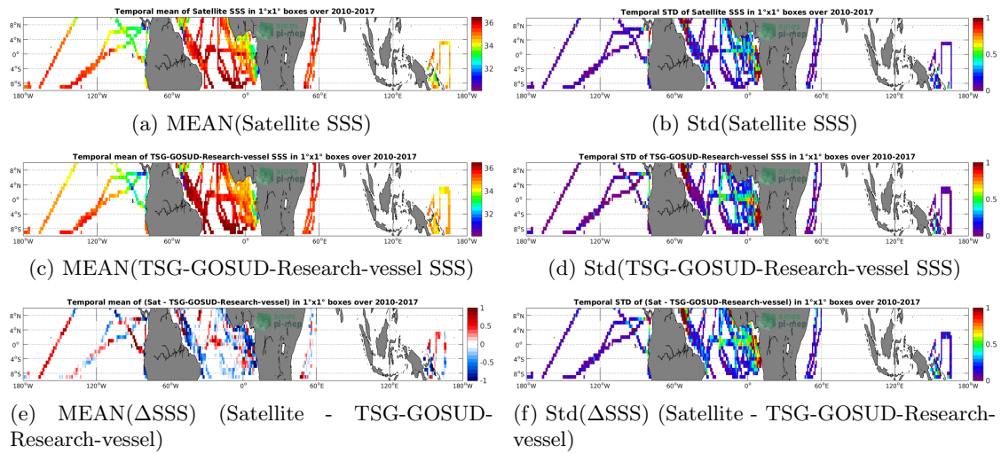
Figure 6: Temporal mean (left) and Std (right) of SSS from SMOS-L3-CATDS-IFREMER-CECOS-V2-MONTHLY-0.25DEG (top), TSG-GOSUD-Research-vessel (middle), and of \Delta SSS (Satellite - TSG-GOSUD-Research-vessel). Only match-up pairs are used to generate these maps.
