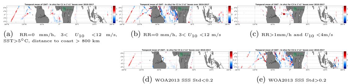
Figure 12: Temporal mean gridded over spatial boxes of size 1^\circ \times 1^\circ of \Delta SSS (SMOS-L3-CATDS-IFREMER-CECOS-V2-MONTHLY-0.25DEG - TSG-GOSUD-Research-vessel) for 5 different subdatasets corresponding to:RR=0 mm/h, 3 < U_{10} < 12 m/s, SST > 5^\circ\text{C} , distance to coast > 800 km (a), RR=0 mm/h, 3 < U_{10} < 12 m/s (b), RR > 1 mm/h and U_{10} < 4 m/s (c), WOA2013 SSS Std < 0.2 (d), WOA2013 SSS Std > 0.2 (e).
