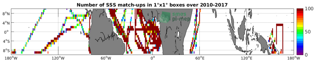
Figure 4: Number of SSS match-ups between TSG-GOSUD-Research-vessel SSS and the SMOS-L3-CATDS-IFREMER-CECOS-V2-MONTHLY-0.25DEG SSS product for the Equatorial Ocean 10N-10S Pi-MEP region over 1°x1° boxes and for the full satellite product period.
