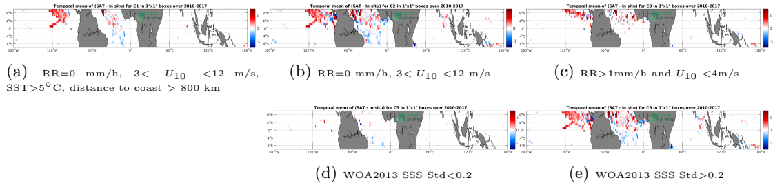
Figure 11: Temporal mean gridded over spatial boxes of size 1^\circ \times 1^\circ of \Delta SSS (SMOS-L3-CATDS-IFREMER-CECOS-V2-MONTHLY-0.25DEG - Surface drifters) for 5 different subdatasets corresponding to: RR=0 mm/h, 3 < U_{10} < 12 m/s, SST >5^\circ\text{C} , distance to coast > 800 km (a), RR=0 mm/h, 3 < U_{10} < 12 m/s (b), RR >1 mm/h and U_{10} < 4 m/s (c), WOA2013 SSS Std <0.2 (d), WOA2013 SSS Std >0.2 (e).
