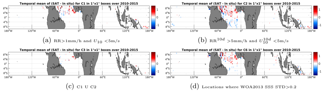
Figure 11: Temporal mean gridded over spatial boxes of size 1^\circ \times 1^\circ of \Delta SSS (SMOS-L3-CATDS-IFREMER-CECOS-V2-MONTHLY-0.25DEG - Surface drifters) for 4 different subdatasets corresponding to: RR > 1\text{mm/h} and U_{10} < 5\text{m/s} (a), RR^{10d} > 5\text{mm/h} and U_{10}^{10d} < 5\text{m/s} (b), C1 U C2 (c), Locations where WOA2013 SSS STD > 0.2 (d).
