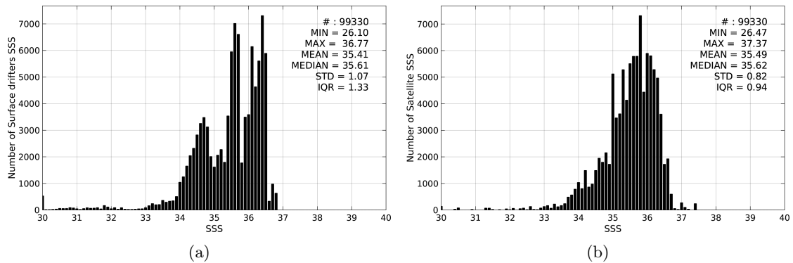
Figure 2: Histograms of SSS from Surface drifters (a) and SMOS-L3-CATDS-IFREMER-CECOS-V2-MONTHLY-0.25DEG (b) considering all match-up pairs per bins of 0.1 over the Equatorial Ocean 10N-10S Pi-MEP region and for the full satellite product period.
