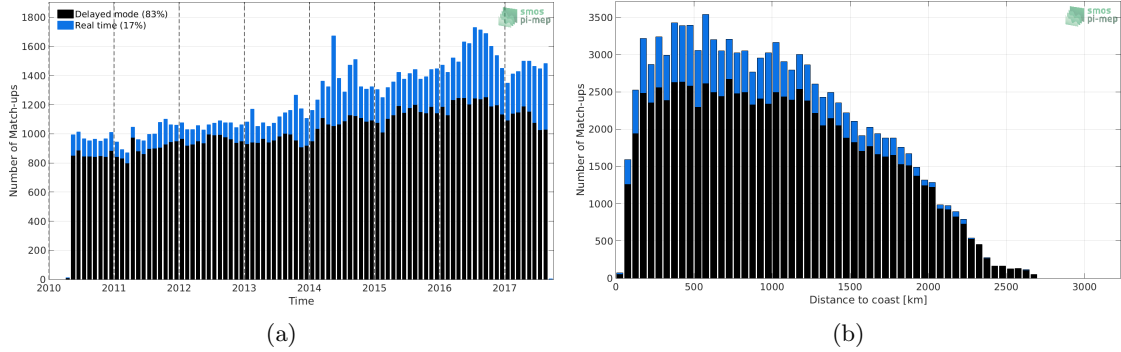
Figure 1: Number of match-ups between Argo and SMOS L3 v2 - Monthly - 0.25 Deg (CATDS-CECOS-IFREMER) SSS as a function of time (a) and as function of the distance to coast (b) over the Equatorial Ocean 10N-10S Pi-MEP region and for the full satellite product period.
