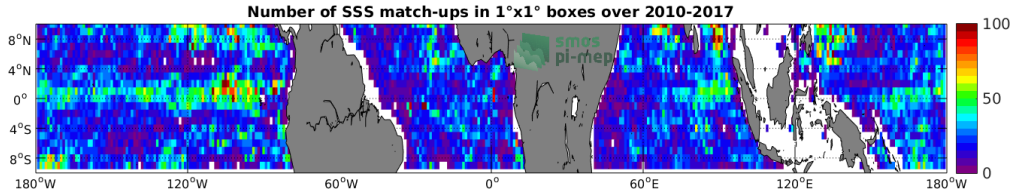
Figure 4: Number of SSS match-ups between Argo SSS and the SMOS L3 v2 - Monthly - 0.25 Deg (CATDS-CECOS-IFREMER) SSS product for the Equatorial Ocean 10N-10S Pi-MEP region over 1°x1° boxes and for the full satellite product period.
