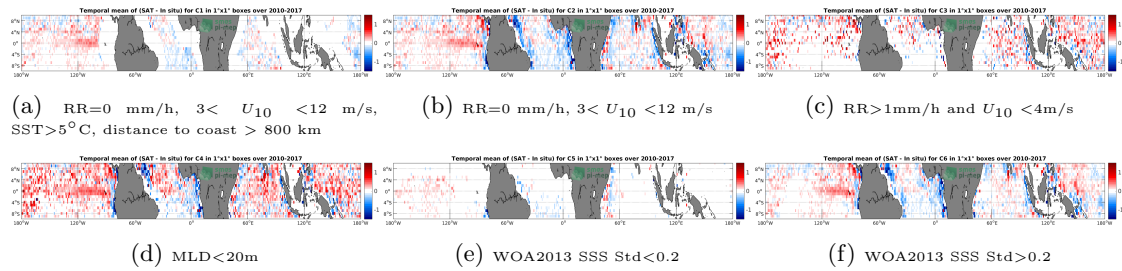
Figure 12: Temporal mean gridded over spatial boxes of size 1^\circ \times 1^\circ of \Delta SSS (SMOS L3 v2 - Monthly - 0.25 Deg (CATDS-CECOS-IFREMER) - Argo) for 6 different subdatasets corresponding to:RR=0 mm/h, 3 < U_{10} < 12 m/s, SST >5^\circ C, distance to coast > 800 km (a), RR=0 mm/h, 3 < U_{10} < 12 m/s (b), RR >1 mm/h and U_{10} < 4 m/s (c),MLD <20 m (d),WOA2013 SSS Std <0.2 (e),WOA2013 SSS Std >0.2 (f).
