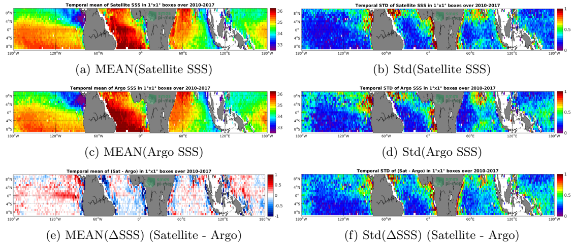
Figure 6: Temporal mean (left) and Std (right) of SSS from SMOS L3 v2 - Monthly - 0.25 Deg (CATDS-CECOS-IFREMER) (top), Argo (middle), and of \Delta SSS (Satellite - Argo). Only match-up pairs are used to generate these maps.
