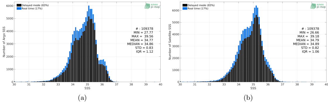
Figure 2: Histograms of SSS from Argo (a) and SMOS L3 v2 - Monthly - 0.25 Deg (CATDS-CECOS-IFREMER) (b) considering all match-up pairs per bins of 0.1 over the Equatorial Ocean 10N-10S Pi-MEP region and for the full satellite product period.
