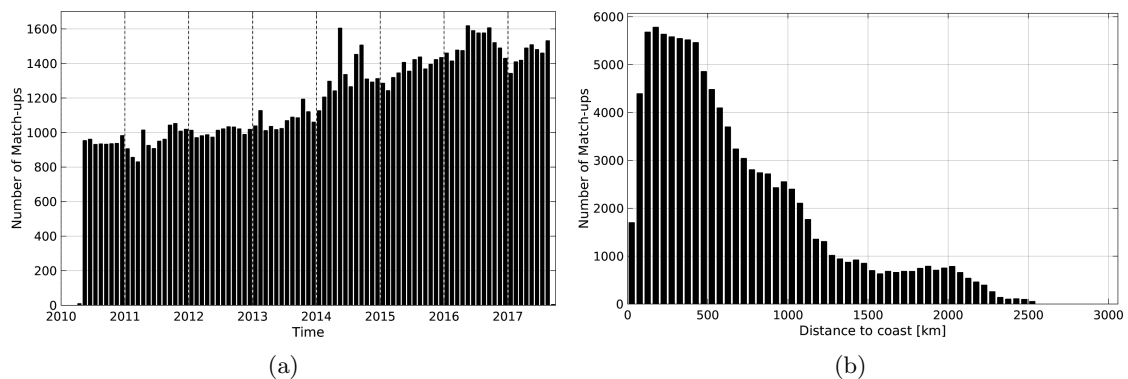
Figure 1: Number of match-ups between Argo and SMOS-L3-CATDS-IFREMER-CECOS-V2-MONTHLY-0.25DEG SSS as a function of time (a) and as function of the distance to coast (b) over the Equatorial Ocean 10N-10S Pi-MEP region and for the full satellite product period.
