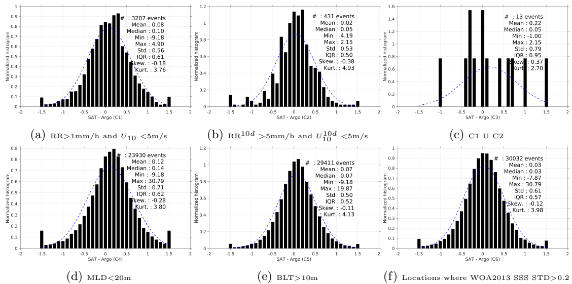
Figure 13: Normalized histogram of \Delta SSS (SMOS-L3-CATDS-IFREMER-CECOS-V2-MONTHLY-0.25DEG - Argo) for 6 different subdatasets corresponding to: RR > 1\text{mm/h} and U_{10} < 5\text{m/s} (a), RR^{10d} > 5\text{mm/h} and U_{10}^{10d} < 5\text{m/s} (b), C1 U C2 (c), MLD < 20\text{m} (d), BLT > 10\text{m} (e), Locations where WOA2013 SSS STD > 0.2 (f).
