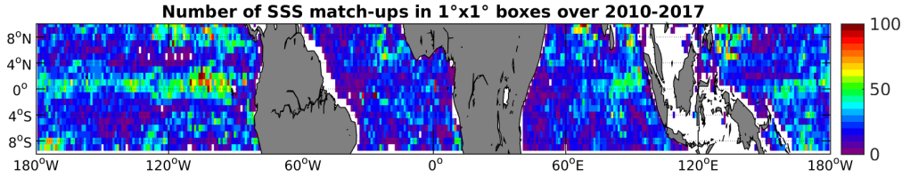
Figure 4: Number of SSS match-ups between Argo SSS and the SMOS-L3-CATDS-IFREMER-CECOS-V2-MONTHLY-0.25DEG SSS product for the Equatorial Ocean 10N-10S Pi-MEP region over 1^\circ \times 1^\circ boxes and for the full satellite product period.
