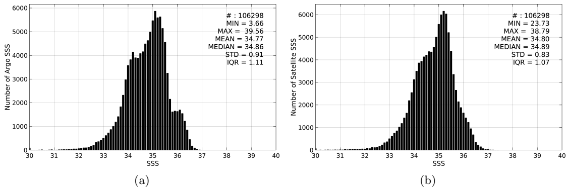
Figure 2: Histograms of SSS from Argo (a) and SMOS-L3-CATDS-IFREMER-CECOS-V2-MONTHLY-0.25DEG (b) considering all match-up pairs per bins of 0.1 over the Equatorial Ocean 10N-10S Pi-MEP region and for the full satellite product period.
