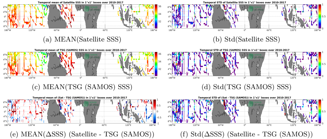
Figure 6: Temporal mean (left) and Std (right) of SSS from SMOS SSS L3 v2 - Daily - 0.5 Deg (CATDS-CECOS-IFREMER) (top), TSG (SAMOS) (middle), and of \Delta SSS (Satellite - TSG (SAMOS)). Only match-up pairs are used to generate these maps.
