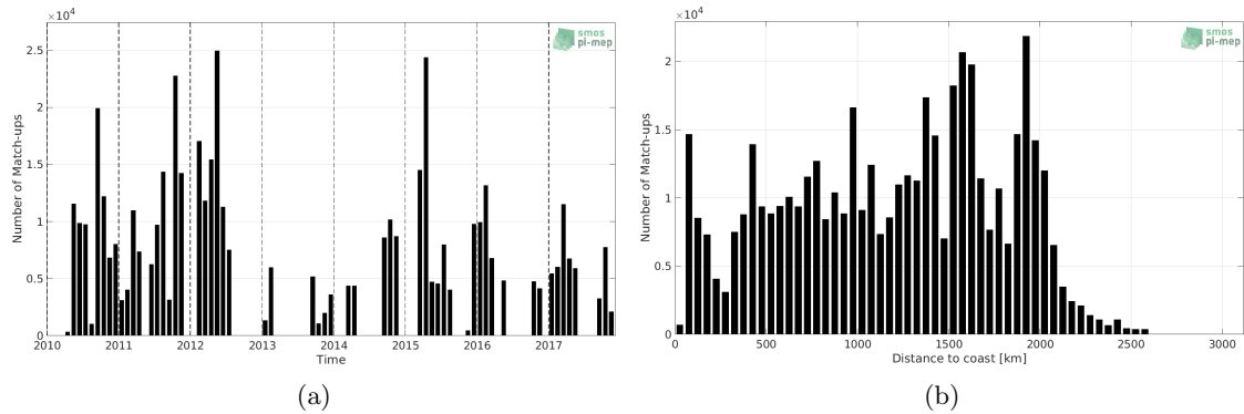
Figure 1: Number of match-ups between TSG (SAMOS) and SMOS SSS L3 v2 - Daily - 0.5 Deg (CATDS-CECOS-IFREMER) SSS as a function of time (a) and as function of the distance to coast (b) over the Equatorial Ocean 10N-10S Pi-MEP region and for the full satellite product period.
