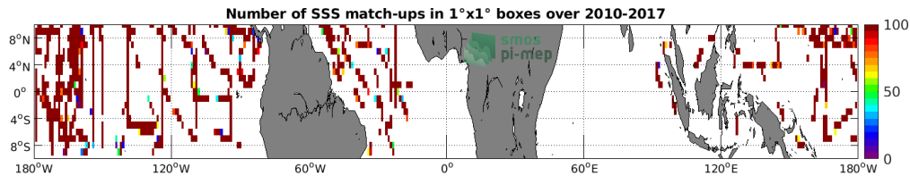
Figure 4: Number of SSS match-ups between TSG (SAMOS) SSS and the SMOS SSS L3 v2 - Daily - 0.5 Deg (CATDS-CECOS-IFREMER) SSS product for the Equatorial Ocean 10N-10S Pi-MEP region over 1^\circ \times 1^\circ boxes and for the full satellite product period.
