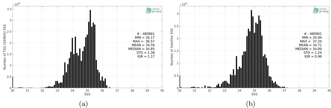
Figure 2: Histograms of SSS from TSG (SAMOS) (a) and SMOS SSS L3 v2 - Daily - 0.5 Deg (CATDS-CECOS-IFREMER) (b) considering all match-up pairs per bins of 0.1 over the Equatorial Ocean 10N-10S Pi-MEP region and for the full satellite product period.
