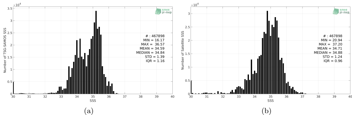
Figure 2: Histograms of SSS from TSG-SAMOS (a) and SMOS L3 v2 - Daily - 0.5 Deg (CATDS-CECOS-IFREMER) (b) considering all match-up pairs per bins of 0.1 over the Equatorial Ocean 10N-10S Pi-MEP region and for the full satellite product period.
