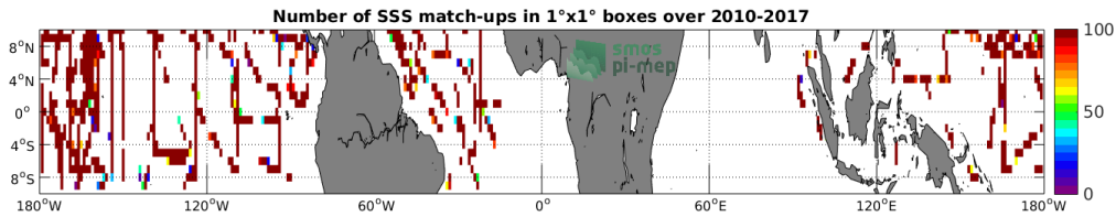
Figure 4: Number of SSS match-ups between TSG-SAMOS SSS and the SMOS L3 v2 - Daily - 0.5 Deg (CATDS-CECOS-IFREMER) SSS product for the Equatorial Ocean 10N-10S Pi-MEP region over 1°x1° boxes and for the full satellite product period.
