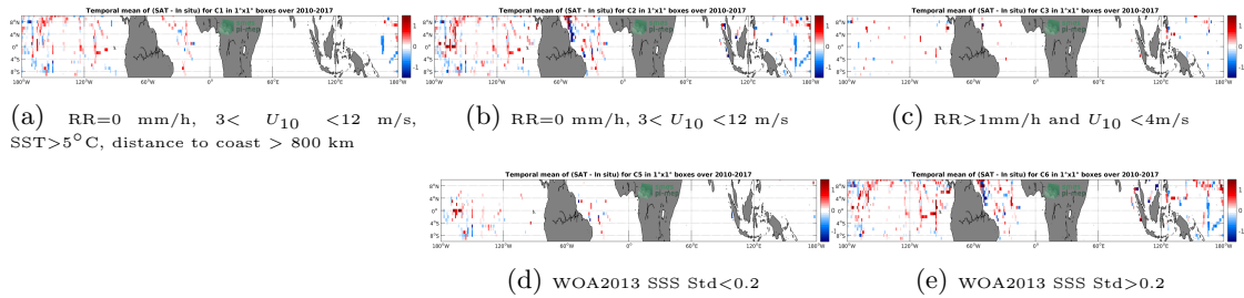
Figure 12: Temporal mean gridded over spatial boxes of size 1°x1° of ΔSSS (SMOS L3 v2 - Daily - 0.5 Deg (CATDS-CECOS-IFREMER) - TSG-SAMOS) for 5 different subdatasets corresponding to: RR=0 mm/h, 3 < U 10 < 12 m/s, SST > 5°C, distance to coast > 800 km (a), RR=0 mm/h, 3 < U 10 < 12 m/s (b), RR > 1mm/h and U 10 < 4m/s (c), WOA2013 SSS Std < 0.2 (d), WOA2013 SSS Std > 0.2 (e).
