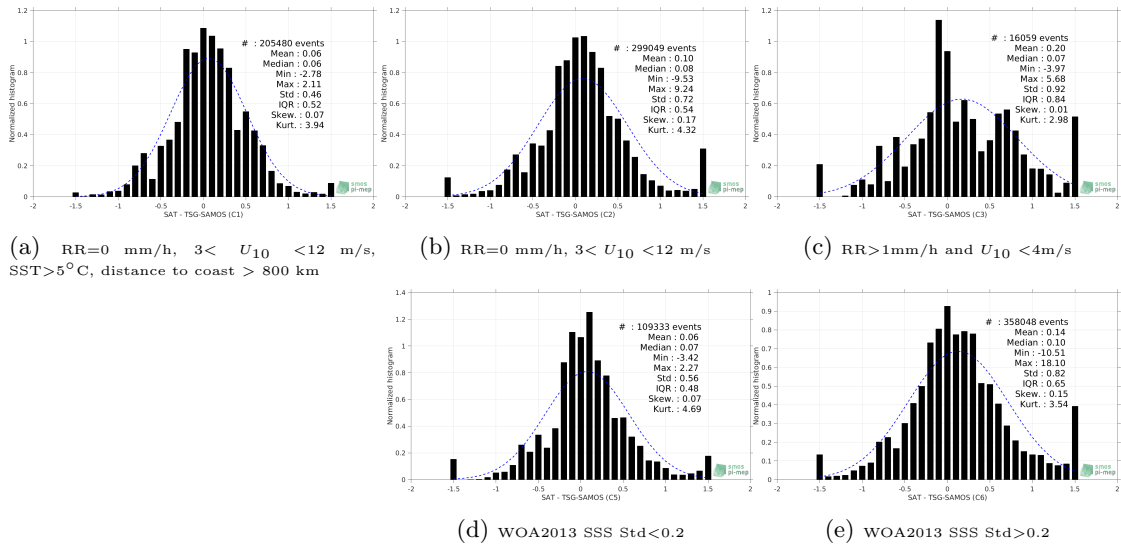
Figure 13: Normalized histogram of ΔSSS (SMOS L3 v2 - Daily - 0.5 Deg (CATDS-CECOS-IFREMER) - TSG-SAMOS) for 5 different subdatasets corresponding to: RR=0 mm/h, 3 < U 10 < 12 m/s, SST > 5°C, distance to coast > 800 km (a), RR=0 mm/h, 3 < U 10 < 12 m/s (b), RR > 1mm/h and U 10 < 4m/s (c), WOA2013 SSS Std < 0.2 (d), WOA2013 SSS Std > 0.2 (e).
