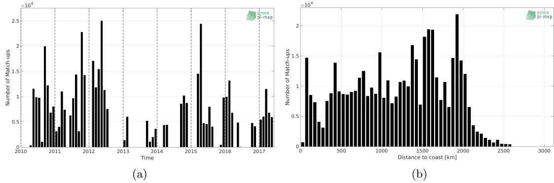
Figure 1: Number of match-ups between TSG-SAMOS and SMOS L3 v2 - Daily - 0.5 Deg (CATDS-CECOS-IFREMER) SSS as a function of time (a) and as function of the distance to coast (b) over the Equatorial Ocean 10N-10S Pi-MEP region and for the full satellite product period.
