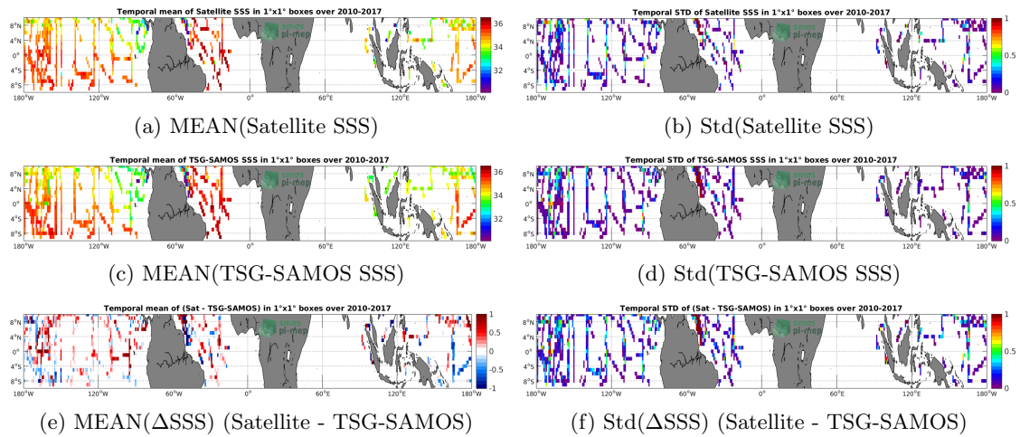
Figure 6: Temporal mean (left) and Std (right) of SSS from SMOS L3 v2 - Daily - 0.5 Deg (CATDS-CECOS-IFREMER) (top), TSG-SAMOS (middle), and of \Delta SSS (Satellite - TSG-SAMOS). Only match-up pairs are used to generate these maps.
