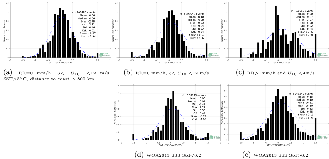
Figure 13: Normalized histogram of \Delta SSS (SMOS-L3-CATDS-CECOS-IFREMER-V2-1DAY-0.5DEG - TSG-SAMOS) for 5 different subdatasets corresponding to: RR=0 mm/h, 3 < U_{10} < 12 m/s, SST >5^\circ\text{C} , distance to coast > 800 km (a), RR=0 mm/h, 3 < U_{10} < 12 m/s (b), RR >1 mm/h and U_{10} < 4 m/s (c), WOA2013 SSS Std <0.2 (d), WOA2013 SSS Std >0.2 (e).
