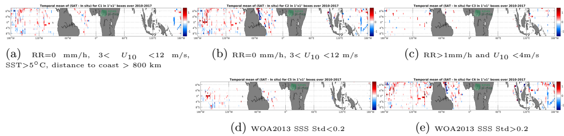
Figure 12: Temporal mean gridded over spatial boxes of size 1^\circ \times 1^\circ of \Delta SSS (SMOS-L3-CATDS-CECOS-IFREMER-V2-1DAY-0.5DEG - TSG-SAMOS) for 5 different subdatasets corresponding to: RR=0 mm/h, 3 < U_{10} < 12 m/s, SST >5^\circ\text{C} , distance to coast > 800 km (a), RR=0 mm/h, 3 < U_{10} < 12 m/s (b), RR >1 mm/h and U_{10} < 4 m/s (c), WOA2013 SSS Std <0.2 (d), WOA2013 SSS Std >0.2 (e).
