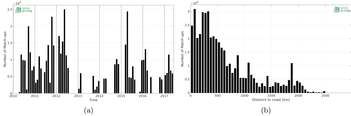
Figure 1: Number of match-ups between TSG-SAMOS and SMOS-L3-CATDS-CECOS-IFREMER-V2-1DAY-0.5DEG SSS as a function of time (a) and as function of the distance to coast (b) over the Equatorial Ocean 10N-10S Pi-MEP region and for the full satellite product period.
