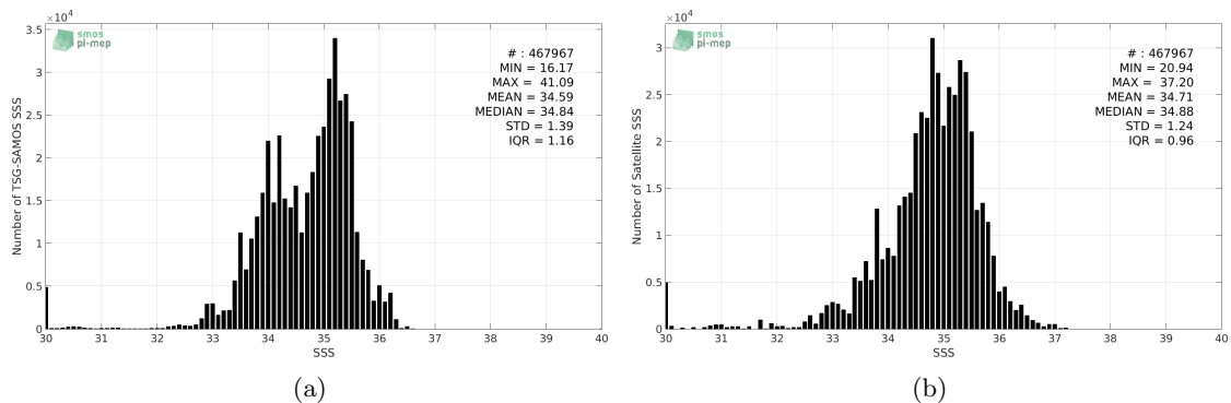
Figure 2: Histograms of SSS from TSG-SAMOS (a) and SMOS-L3-CATDS-CECOS-IFREMER-V2-1DAY-0.5DEG (b) considering all match-up pairs per bins of 0.1 over the Equatorial Ocean 10N-10S Pi-MEP region and for the full satellite product period.
