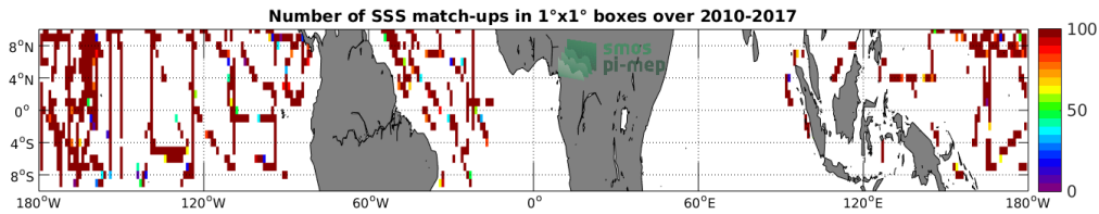
Figure 4: Number of SSS match-ups between TSG-SAMOS SSS and the SMOS-L3-CATDS-CECOS-IFREMER-V2-1DAY-0.5DEG SSS product for the Equatorial Ocean 10N-10S Pi-MEP region over 1°x1° boxes and for the full satellite product period.
