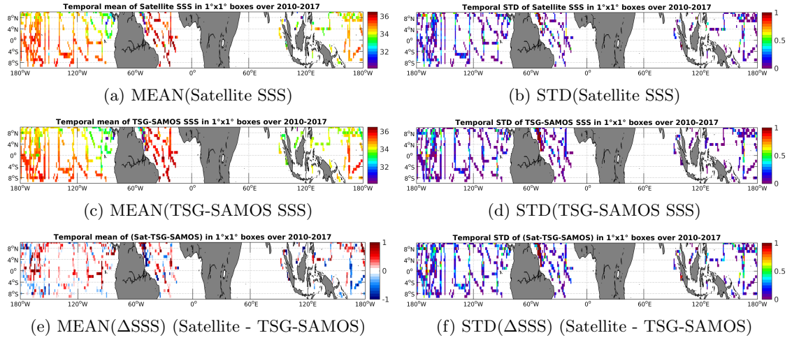
Figure 6: Temporal mean (left) and STD (right) of SSS from SMOS-L3-CATDS-CECOS-IFREMER-V2-1DAY-0.5deg (top), TSG-SAMOS (middle), and of \Delta SSS (Satellite - TSG-SAMOS). Only match-up pairs are used to generate these maps.
