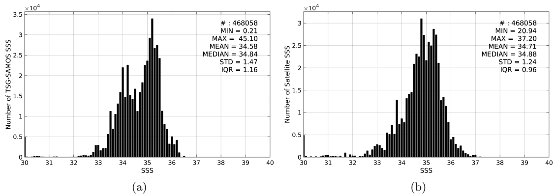
Figure 2: Histograms of SSS from TSG-SAMOS (a) and SMOS-L3-CATDS-CECOS-IFREMER-V2-1DAY-0.5deg (b) considering all match-up pairs per bins of 0.1 over the Equatorial Ocean 10N-10S Pi-MEP region and for the full satellite product period.
