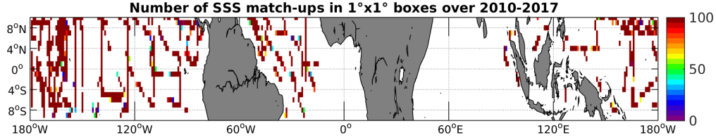
Figure 4: Number of SSS match-ups between TSG-SAMOS SSS and the SMOS-L3-CATDS-CECOS-IFREMER-V2-1DAY-0.5deg SSS product for the Equatorial Ocean 10N-10S Pi-MEP region over 1^\circ \times 1^\circ boxes and for the full satellite product period.
