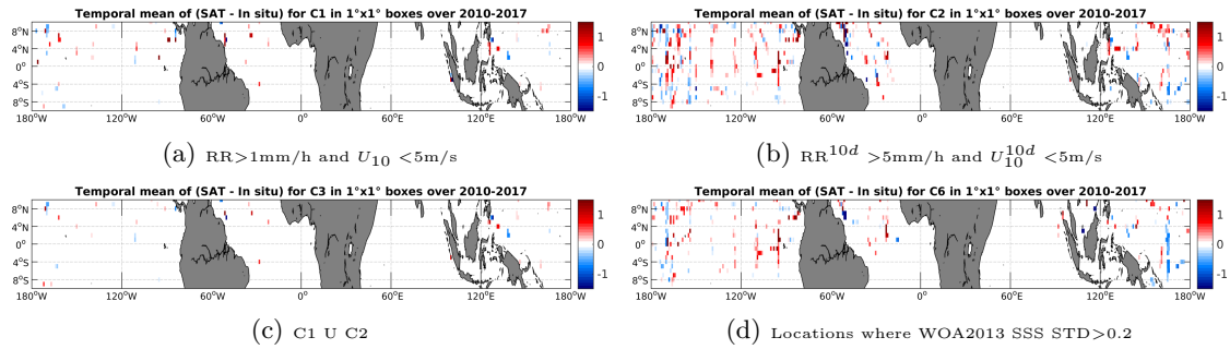
Figure 12: Temporal mean gridded over spatial boxes of size 1^\circ \times 1^\circ of \Delta SSS (SMOS-L3-CATDS-CECOS-IFREMER-V2-1DAY-0.5deg - TSG-SAMOS) for 4 different subdatasets corresponding to: RR > 1\text{mm/h} and U_{10} < 5\text{m/s} (a), RR^{10d} > 5\text{mm/h} and U_{10}^{10d} < 5\text{m/s} (b), C1 U C2 (c), Locations where WOA2013 SSS STD > 0.2 (d).
