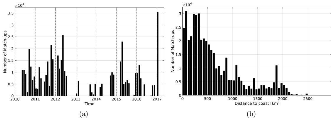
Figure 1: Number of match-ups between TSG-SAMOS and SMOS-L3-CATDS-CECOS-IFREMER-V2-1DAY-0.5deg SSS as a function of time (a) and as function of the distance to coast (b) over the Equatorial Ocean 10N-10S Pi-MEP region and for the full satellite product period.
