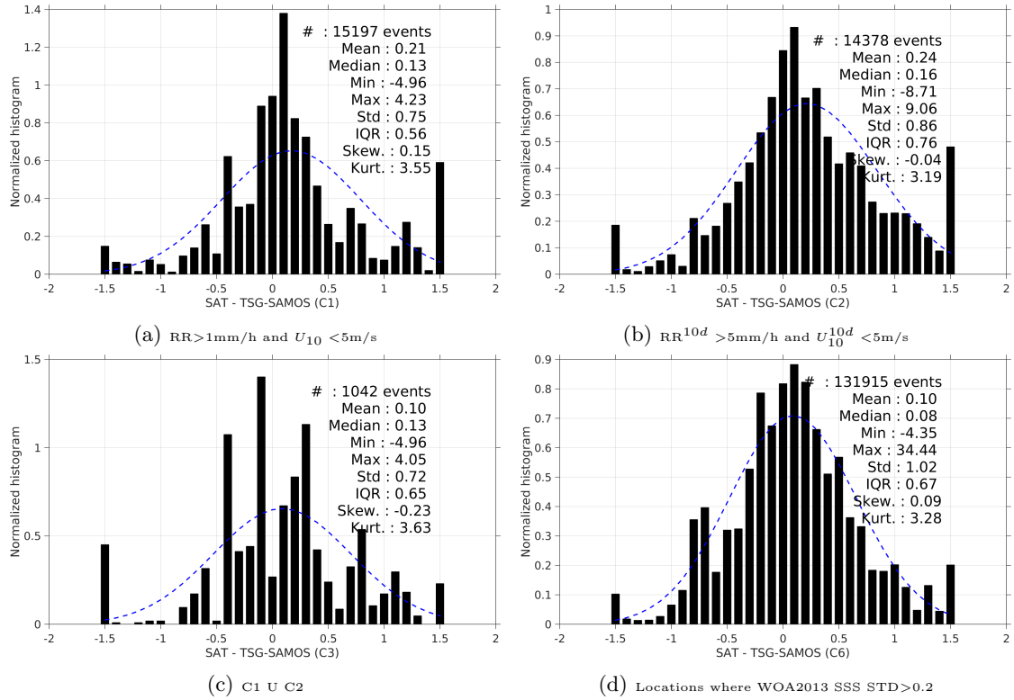
Figure 13: Normalized histogram of \Delta SSS (SMOS-L3-CATDS-CECOS-IFREMER-V2-1DAY-0.5deg - TSG-SAMOS) for 6 different subdatasets corresponding to: RR > 1\text{mm/h} and U_{10} < 5\text{m/s} (a), RR^{10d} > 5\text{mm/h} and U_{10}^{10d} < 5\text{m/s} (b), C1 U C2 (c), Locations where WOA2013 SSS STD > 0.2 (d).
