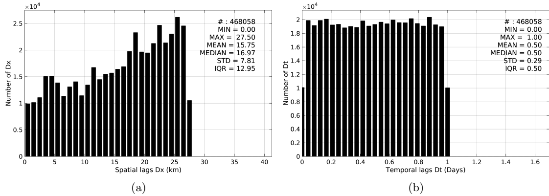
Figure 5: Histograms of the spatial (a) and temporal (b) lags between the time of the TSG-SAMOS measurements and the date of the corresponding SMOS-L3-CATDS-CECOS-IFREMER-V2-1DAY-0.5deg SSS product.
