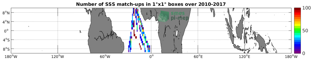
Figure 4: Number of SSS match-ups between TSG (Polarstern) SSS and the SMOS SSS L3 v2 - Daily - 0.5 Deg (CATDS-CECOS-IFREMER) SSS product for the Equatorial Ocean 10N-10S Pi-MEP region over 1°x1° boxes and for the full satellite product period.
