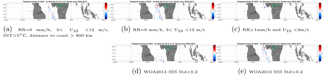
Figure 12: Temporal mean gridded over spatial boxes of size 1^{\circ}\times 1^{\circ} of \Delta\text{SSS} (SMOS L3 v2 - Daily - 0.5 Deg (CATDS-CECOS-IFREMER) - TSG-POLARSTERN) for 5 different subdatasets corresponding to:RR=0 mm/h, 3 < U_{10} < 12 m/s, SST >5^{\circ}\text{C} , distance to coast > 800 km (a), RR=0 mm/h, 3 < U_{10} < 12 m/s (b), RR >1 mm/h and U_{10} < 4 m/s (c), WOA2013 SSS Std <0.2 (d), WOA2013 SSS Std >0.2 (e).
