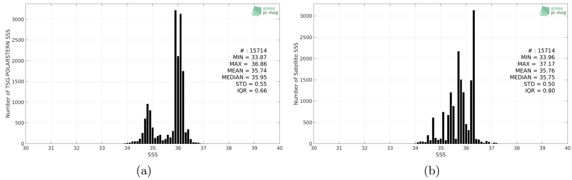
Figure 2: Histograms of SSS from TSG-POLARSTERN (a) and SMOS L3 v2 - Daily - 0.5 Deg (CATDS-CECOS-IFREMER) (b) considering all match-up pairs per bins of 0.1 over the Equatorial Ocean 10N-10S Pi-MEP region and for the full satellite product period.
