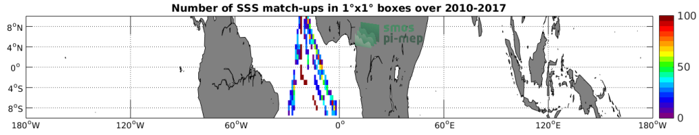
Figure 4: Number of SSS match-ups between TSG-POLARSTERN SSS and the SMOS L3 v2 - Daily - 0.5 Deg (CATDS-CECOS-IFREMER) SSS product for the Equatorial Ocean 10N-10S Pi-MEP region over 1°x1° boxes and for the full satellite product period.
