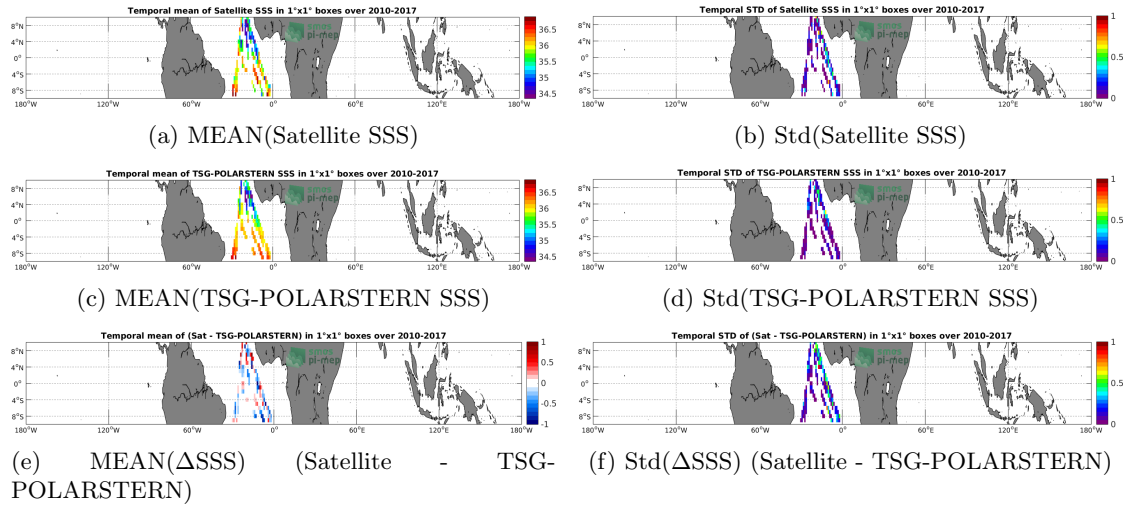
Figure 6: Temporal mean (left) and Std (right) of SSS from SMOS L3 v2 - Daily - 0.5 Deg (CATDS-CECOS-IFREMER) (top), TSG-POLARSTERN (middle), and of \Delta SSS (Satellite - TSG-POLARSTERN). Only match-up pairs are used to generate these maps.
