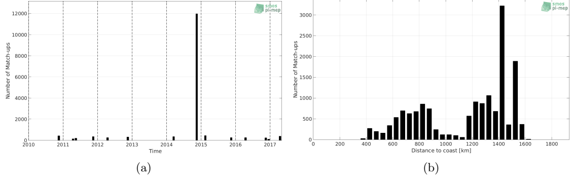
Figure 1: Number of match-ups between TSG-POLARSTERN and SMOS L3 v2 - Daily - 0.5 Deg (CATDS-CECOS-IFREMER) SSS as a function of time (a) and as function of the distance to coast (b) over the Equatorial Ocean 10N-10S Pi-MEP region and for the full satellite product period.
