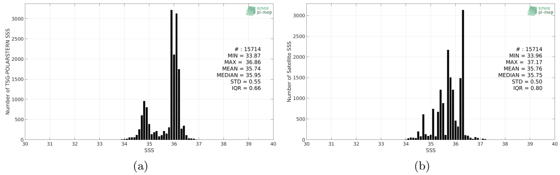
Figure 2: Histograms of SSS from TSG-POLARSTERN (a) and SMOS-L3-CATDS-CECOS-IFREMER-V2-1DAY-0.5DEG (b) considering all match-up pairs per bins of 0.1 over the Equatorial Ocean 10N-10S Pi-MEP region and for the full satellite product period.
