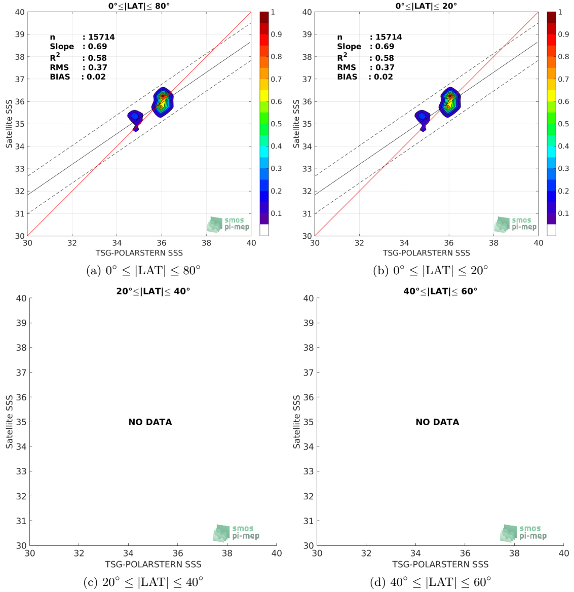
Figure 9: Contour maps of the concentration of SMOS-L3-CATDS-CECOS-IFREMER-V2-1DAY-0.5DEG SSS (y-axis) versus TSG-POLARSTERN SSS (x-axis) at match-up pairs for different latitude bands. For each plot, the red line shows x=y . The black thin and dashed lines indicate a linear fit through the data cloud and the \pm 95\% confidence levels, respectively. The number match-up pairs n , the slope and R^2 coefficient of the linear fit, the root mean square (RMS) and the mean bias between satellite and in situ data are indicated for each latitude band in each plots.
