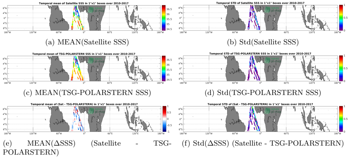
Figure 6: Temporal mean (left) and Std (right) of SSS from SMOS-L3-CATDS-CECOS-IFREMER-V2-1DAY-0.5DEG (top), TSG-POLARSTERN (middle), and of \Delta SSS (Satellite - TSG-POLARSTERN). Only match-up pairs are used to generate these maps.
