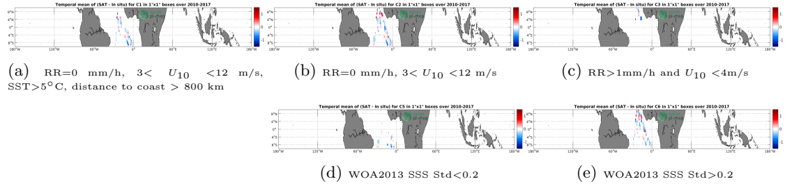
Figure 12: Temporal mean gridded over spatial boxes of size 1^\circ \times 1^\circ of \Delta SSS (SMOS-L3-CATDS-CECOS-IFREMER-V2-1DAY-0.5DEG - TSG-POLARSTERN) for 5 different subdatasets corresponding to: RR=0 mm/h, 3 < U_{10} < 12 m/s, SST > 5^\circ C , distance to coast > 800 km (a), RR=0 mm/h, 3 < U_{10} < 12 m/s (b), RR > 1 mm/h and U_{10} < 4 m/s (c), WOA2013 SSS Std < 0.2 (d), WOA2013 SSS Std > 0.2 (e).
