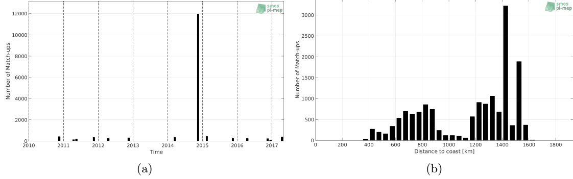
Figure 1: Number of match-ups between TSG-POLARSTERN and SMOS-L3-CATDS-CECOS-IFREMER-V2-1DAY-0.5DEG SSS as a function of time (a) and as function of the distance to coast (b) over the Equatorial Ocean 10N-10S Pi-MEP region and for the full satellite product period.
