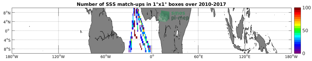
Figure 4: Number of SSS match-ups between TSG-POLARSTERN SSS and the SMOS-L3-CATDS-CECOS-IFREMER-V2-1DAY-0.5DEG SSS product for the Equatorial Ocean 10N-10S Pi-MEP region over 1^\circ \times 1^\circ boxes and for the full satellite product period.
