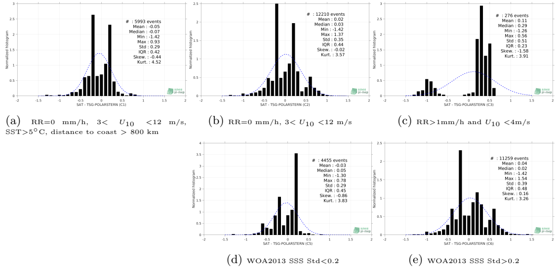
Figure 13: Normalized histogram of \Delta SSS (SMOS-L3-CATDS-CECOS-IFREMER-V2-1DAY-0.5DEG - TSG-POLARSTERN) for 5 different subdatasets corresponding to: RR=0 mm/h, 3 < U_{10} < 12 m/s, SST > 5^\circ C , distance to coast > 800 km (a), RR=0 mm/h, 3 < U_{10} < 12 m/s (b), RR > 1 mm/h and U_{10} < 4 m/s (c), WOA2013 SSS Std < 0.2 (d), WOA2013 SSS Std > 0.2 (e).
