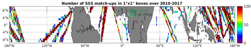
Figure 4: Number of SSS match-ups between TSG (LEGOS-DM) SSS and the SMOS SSS L3 v2 - Daily - 0.5 Deg (CATDS-CECOS-IFREMER) SSS product for the Equatorial Ocean 10N-10S Pi-MEP region over 1^\circ \times 1^\circ boxes and for the full satellite product period.
