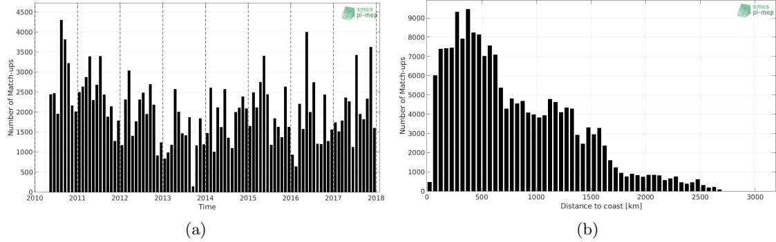
Figure 1: Number of match-ups between TSG (LEGOS-DM) and SMOS SSS L3 v2 - Daily - 0.5 Deg (CATDS-CECOS-IFREMER) SSS as a function of time (a) and as function of the distance to coast (b) over the Equatorial Ocean 10N-10S Pi-MEP region and for the full satellite product period.
