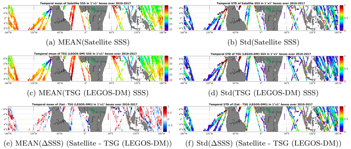
Figure 6: Temporal mean (left) and Std (right) of SSS from SMOS SSS L3 v2 - Daily - 0.5 Deg (CATDS-CECOS-IFREMER) (top), TSG (LEGOS-DM) (middle), and of \Delta SSS (Satellite - TSG (LEGOS-DM)). Only match-up pairs are used to generate these maps.
