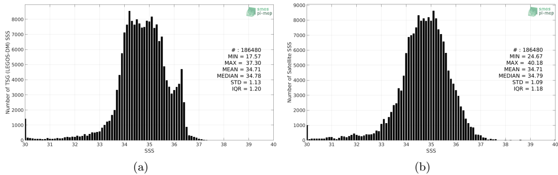
Figure 2: Histograms of SSS from TSG (LEGOS-DM) (a) and SMOS SSS L3 v2 - Daily - 0.5 Deg (CATDS-CECOS-IFREMER) (b) considering all match-up pairs per bins of 0.1 over the Equatorial Ocean 10N-10S Pi-MEP region and for the full satellite product period.
