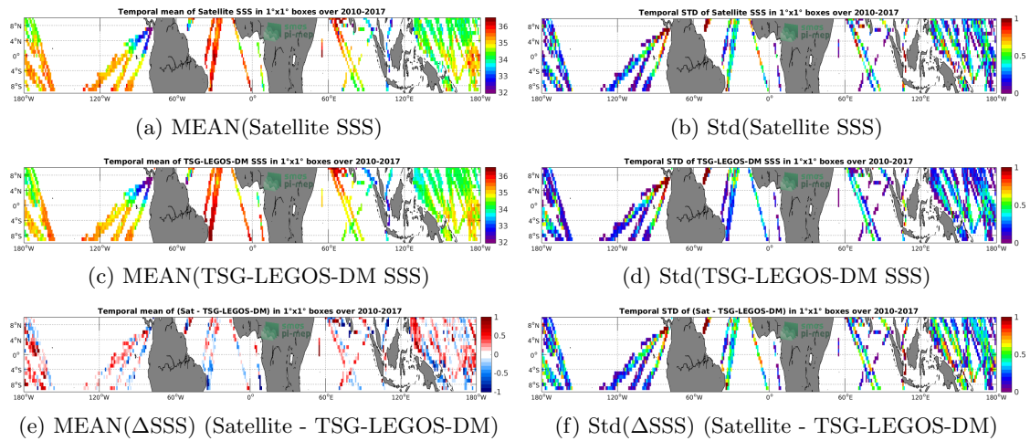
Figure 6: Temporal mean (left) and Std (right) of SSS from SMOS L3 v2 - Daily - 0.5 Deg (CATDS-CECOS-IFREMER) (top), TSG-LEGOS-DM (middle), and of \Delta SSS (Satellite - TSG-LEGOS-DM). Only match-up pairs are used to generate these maps.
