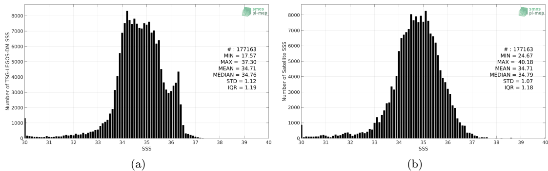
Figure 2: Histograms of SSS from TSG-LEGOS-DM (a) and SMOS L3 v2 - Daily - 0.5 Deg (CATDS-CECOS-IFREMER) (b) considering all match-up pairs per bins of 0.1 over the Equatorial Ocean 10N-10S Pi-MEP region and for the full satellite product period.
