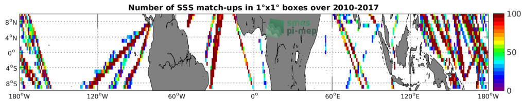
Figure 4: Number of SSS match-ups between TSG-LEGOS-DM SSS and the SMOS L3 v2 - Daily - 0.5 Deg (CATDS-CECOS-IFREMER) SSS product for the Equatorial Ocean 10N-10S Pi-MEP region over 1^\circ \times 1^\circ boxes and for the full satellite product period.
