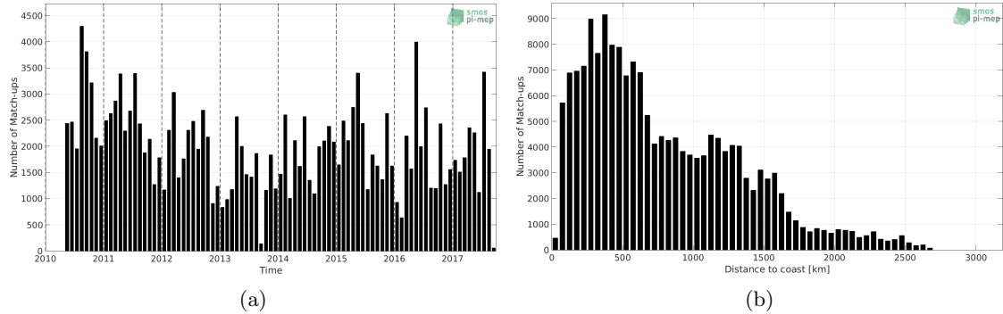
Figure 1: Number of match-ups between TSG-LEGOS-DM and SMOS L3 v2 - Daily - 0.5 Deg (CATDS-CECOS-IFREMER) SSS as a function of time (a) and as function of the distance to coast (b) over the Equatorial Ocean 10N-10S Pi-MEP region and for the full satellite product period.
