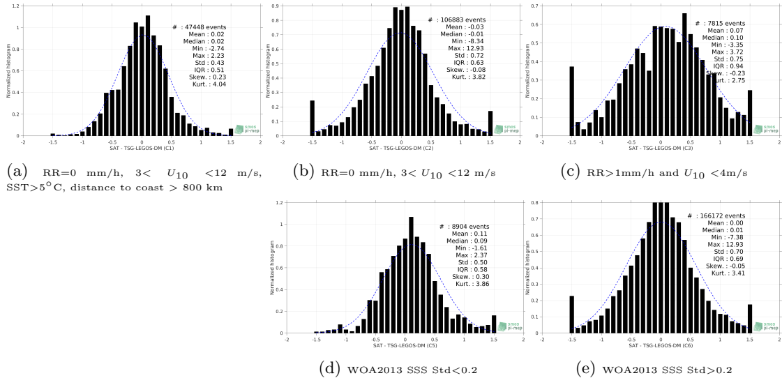
Figure 13: Normalized histogram of ΔSSS (SMOS-L3-CATDS-CECOS-IFREMER-V2-1DAY-0.5DEG - TSG-LEGOS-DM) for 5 different subdatasets corresponding to: RR=0 mm/h, 3 < U 10 < 12 m/s, SST>5°C, distance to coast > 800 km (a), RR=0 mm/h, 3 < U 10 < 12 m/s (b), RR>1mm/h and U 10 < 4m/s (c), WOA2013 SSS Std<0.2 (d), WOA2013 SSS Std>0.2 (e).
