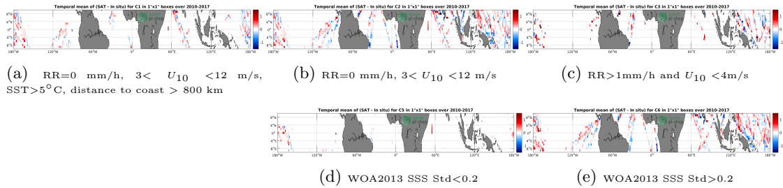
Figure 12: Temporal mean gridded over spatial boxes of size 1°x1° of ΔSSS (SMOS-L3-CATDS-CECOS-IFREMER-V2-1DAY-0.5DEG - TSG-LEGOS-DM) for 5 different subdatasets corresponding to:RR=0 mm/h, 3 < U 10 < 12 m/s, SST>5°C, distance to coast > 800 km (a), RR=0 mm/h, 3 < U 10 < 12 m/s (b), RR>1mm/h and U 10 < 4m/s (c), WOA2013 SSS Std<0.2 (d), WOA2013 SSS Std>0.2 (e).
