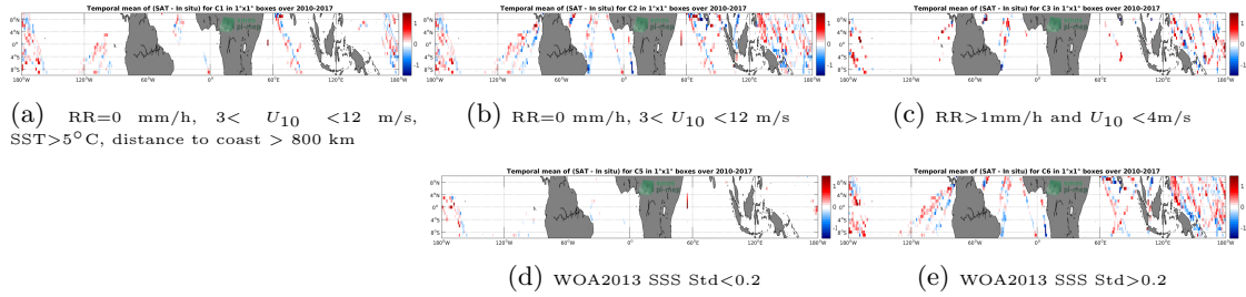
Figure 12: Temporal mean gridded over spatial boxes of size 1^\circ \times 1^\circ of \Delta SSS (SMOS-L3-CATDS-CECOS-IFREMER-V2-1DAY-0.5DEG - TSG-LEGOS-DM) for 5 different subdatasets corresponding to:RR=0 mm/h, 3 < U_{10} < 12 m/s, SST >5^\circ C, distance to coast > 800 km (a), RR=0 mm/h, 3 < U_{10} < 12 m/s (b), RR >1 mm/h and U_{10} < 4 m/s (c), WOA2013 SSS Std <0.2 (d), WOA2013 SSS Std >0.2 (e).
