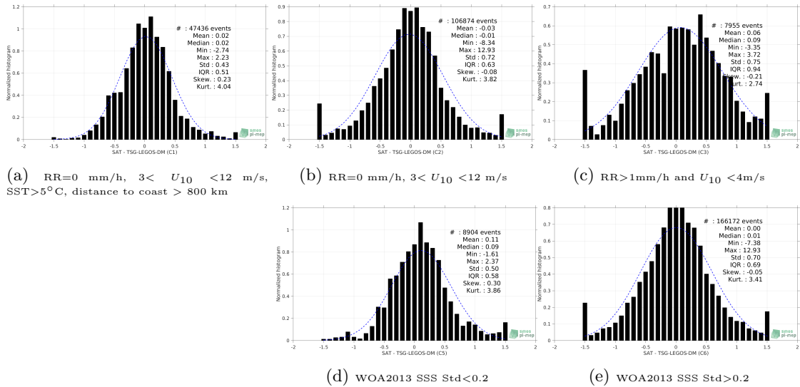
Figure 13: Normalized histogram of \Delta SSS (SMOS-L3-CATDS-CECOS-IFREMER-V2-1DAY-0.5DEG - TSG-LEGOS-DM) for 5 different subdatasets corresponding to: RR=0 mm/h, 3 < U_{10} < 12 m/s, SST >5^\circ C, distance to coast > 800 km (a), RR=0 mm/h, 3 < U_{10} < 12 m/s (b), RR >1 mm/h and U_{10} < 4 m/s (c), WOA2013 SSS Std <0.2 (d), WOA2013 SSS Std >0.2 (e).
