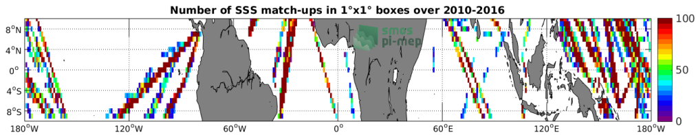
Figure 4: Number of SSS match-ups between TSG-LEGOS-DM SSS and the SMOS-L3-CATDS-CECOS-IFREMER-V2-1DAY-0.5DEG SSS product for the Equatorial Ocean 10N-10S Pi-MEP region over 1°x1° boxes and for the full satellite product period.
