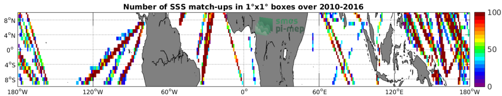
Figure 4: Number of SSS match-ups between TSG-LEGOS-DM SSS and the SMOS-L3-CATDS-CECOS-IFREMER-V2-1DAY-0.5DEG SSS product for the Equatorial Ocean 10N-10S Pi-MEP region over 1^\circ \times 1^\circ boxes and for the full satellite product period.
