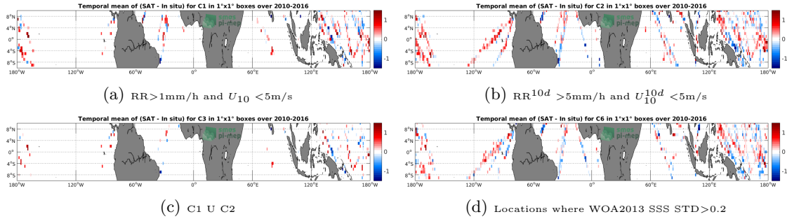
Figure 12: Temporal mean gridded over spatial boxes of size 1^\circ \times 1^\circ of \Delta SSS (SMOS-L3-CATDS-CECOS-IFREMER-V2-1DAY-0.5DEG - TSG-LEGOS-DM) for 4 different subdatasets corresponding to: RR>1mm/h and U_{10} < 5\text{m/s} (a), RR^{10d} > 5\text{mm/h} and U_{10}^{10d} < 5\text{m/s} (b), C1 U C2 (c), Locations where WOA2013 SSS STD>0.2 (d).
