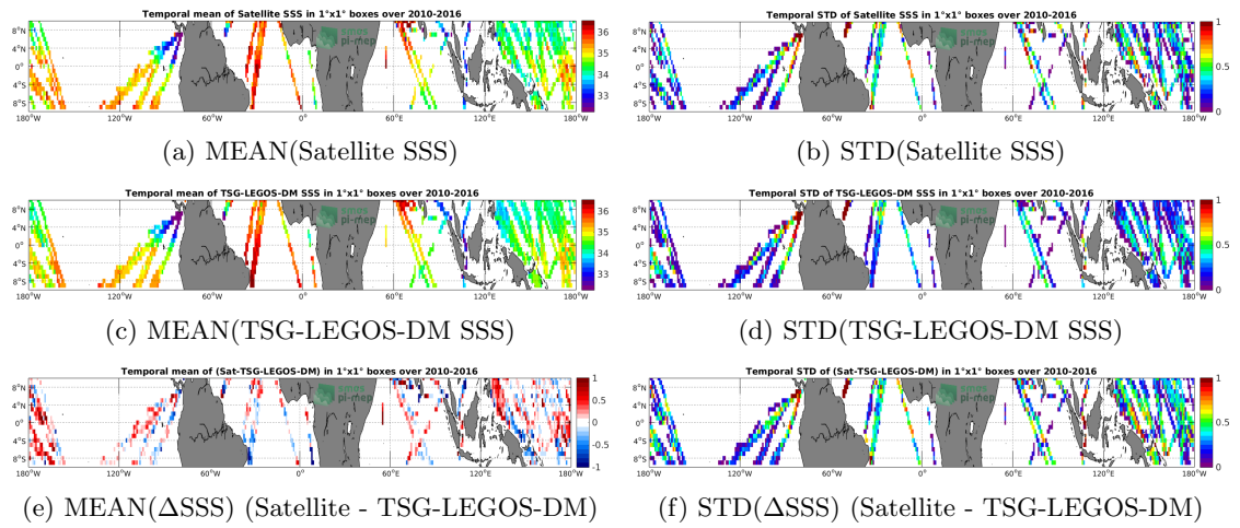
Figure 6: Temporal mean (left) and STD (right) of SSS from SMOS-L3-CATDS-CECOS-IFREMER-V2-1DAY-0.5DEG (top), TSG-LEGOS-DM (middle), and of \Delta SSS (Satellite - TSG-LEGOS-DM). Only match-up pairs are used to generate these maps.
