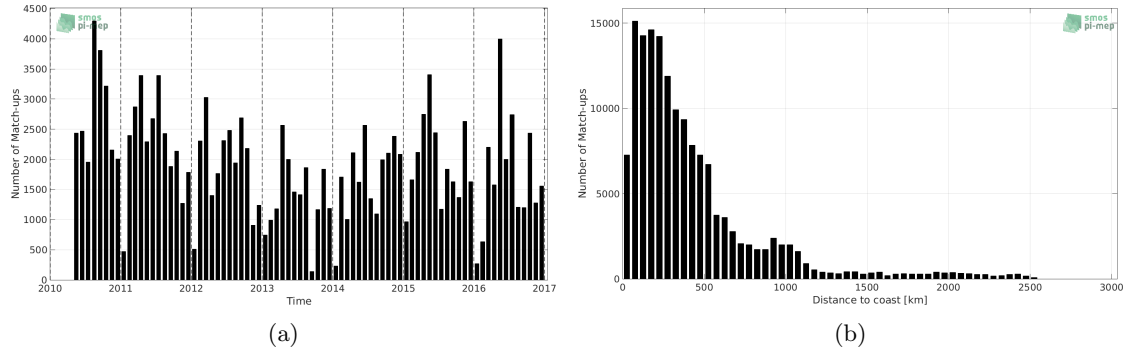
Figure 1: Number of match-ups between TSG-LEGOS-DM and SMOS-L3-CATDS-CECOS-IFREMER-V2-1DAY-0.5DEG SSS as a function of time (a) and as function of the distance to coast (b) over the Equatorial Ocean 10N-10S Pi-MEP region and for the full satellite product period.
