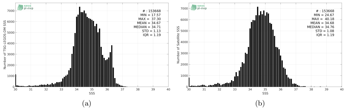
Figure 2: Histograms of SSS from TSG-LEGOS-DM (a) and SMOS-L3-CATDS-CECOS-IFREMER-V2-1DAY-0.5DEG (b) considering all match-up pairs per bins of 0.1 over the Equatorial Ocean 10N-10S Pi-MEP region and for the full satellite product period.
