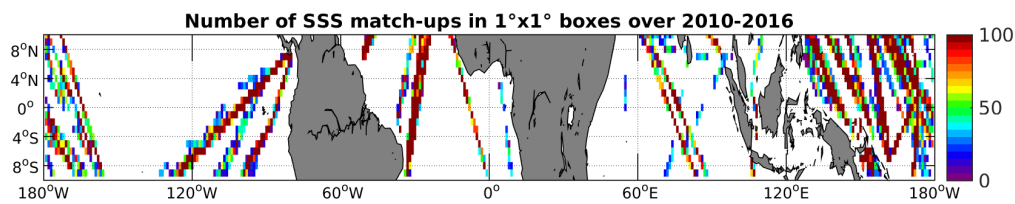
Figure 4: Number of SSS match-ups between TSG-LEGOS-DM SSS and the SMOS-L3-CATDS-CECOS-IFREMER-V2-1DAY-0.5DEG SSS product for the Equatorial Ocean 10N-10S Pi-MEP region over 1^\circ \times 1^\circ boxes and for the full satellite product period.
