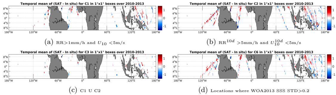
Figure 12: Temporal mean gridded over spatial boxes of size 1^\circ \times 1^\circ of \Delta SSS (SMOS-L3-CATDS-CECOS-IFREMER-V2-1DAY-0.5deg - TSG-LEGOS-DM) for 4 different subdatasets corresponding to: RR > 1\text{mm/h} and U_{10} < 5\text{m/s} (a), RR^{10d} > 5\text{mm/h} and U_{10}^{10d} < 5\text{m/s} (b), C1 U C2 (c), Locations where WOA2013 SSS STD > 0.2 (d).
