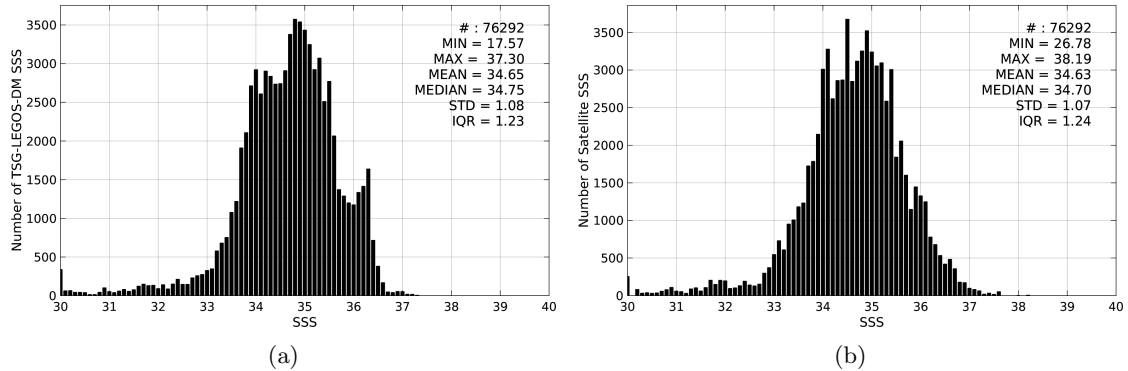
Figure 2: Histograms of SSS from TSG-LEGOS-DM (a) and SMOS-L3-CATDS-CECOS-IFREMER-V2-1DAY-0.5deg (b) considering all match-up pairs per bins of 0.1 over the Equatorial Ocean 10N-10S Pi-MEP region and for the full satellite product period.
