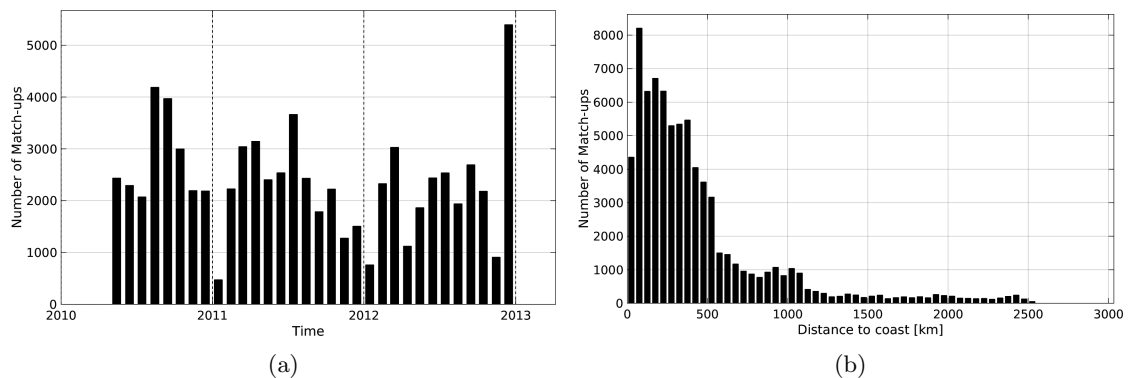
Figure 1: Number of match-ups between TSG-LEGOS-DM and SMOS-L3-CATDS-CECOS-IFREMER-V2-1DAY-0.5deg SSS as a function of time (a) and as function of the distance to coast (b) over the Equatorial Ocean 10N-10S Pi-MEP region and for the full satellite product period.
