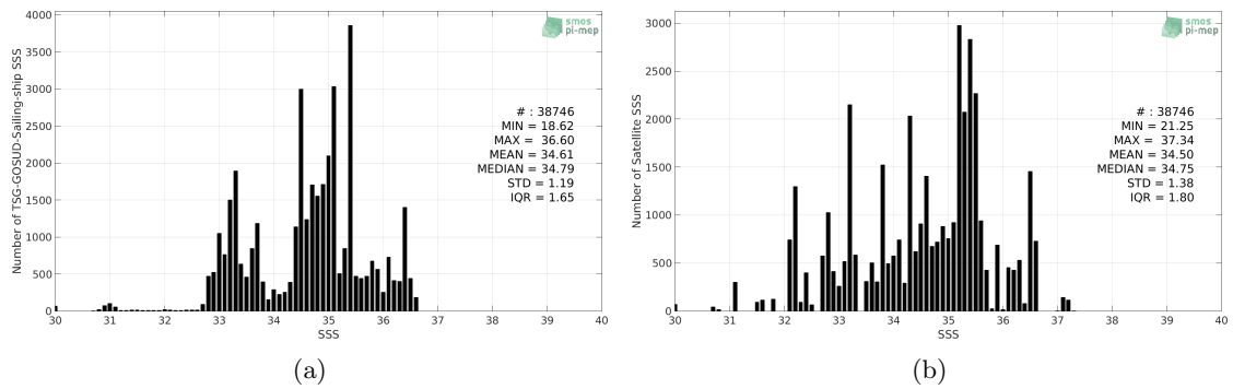
Figure 2: Histograms of SSS from TSG-GOSUD-Sailing-ship (a) and SMOS L3 v2 - Daily - 0.5 Deg (CATDS-CECOS-IFREMER) (b) considering all match-up pairs per bins of 0.1 over the Equatorial Ocean 10N-10S Pi-MEP region and for the full satellite product period.
