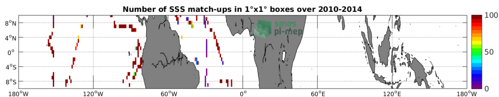
Figure 4: Number of SSS match-ups between TSG-GOSUD-Sailing-ship SSS and the SMOS L3 v2 - Daily - 0.5 Deg (CATDS-CECOS-IFREMER) SSS product for the Equatorial Ocean 10N-10S Pi-MEP region over 1^\circ \times 1^\circ boxes and for the full satellite product period.
