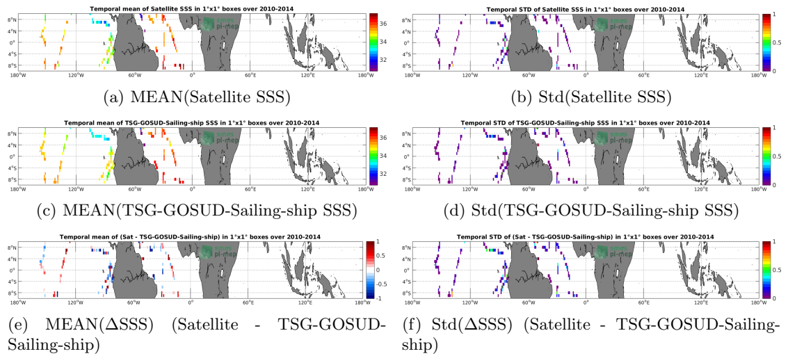
Figure 6: Temporal mean (left) and Std (right) of SSS from SMOS L3 v2 - Daily - 0.5 Deg (CATDS-CECOS-IFREMER) (top), TSG-GOSUD-Sailing-ship (middle), and of \Delta SSS (Satellite - TSG-GOSUD-Sailing-ship). Only match-up pairs are used to generate these maps.
