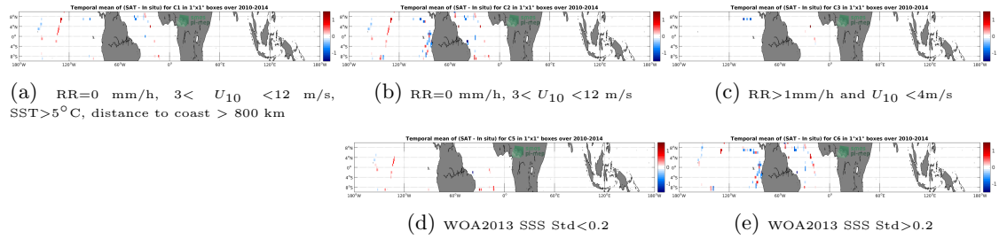
Figure 12: Temporal mean gridded over spatial boxes of size 1^{\circ}\times 1^{\circ} of \Delta SSS (SMOS L3 v2 - Daily - 0.5 Deg (CATDS-CECOS-IFREMER) - TSG-GOSUD-Sailing-ship) for 5 different subdatasets corresponding to:RR=0 mm/h, 3 < U_{10} < 12 m/s, SST >5^{\circ}\text{C} , distance to coast > 800 km (a), RR=0 mm/h, 3 < U_{10} < 12 m/s (b), RR >1 mm/h and U_{10} < 4 m/s (c), WOA2013 SSS Std <0.2 (d), WOA2013 SSS Std >0.2 (e).
