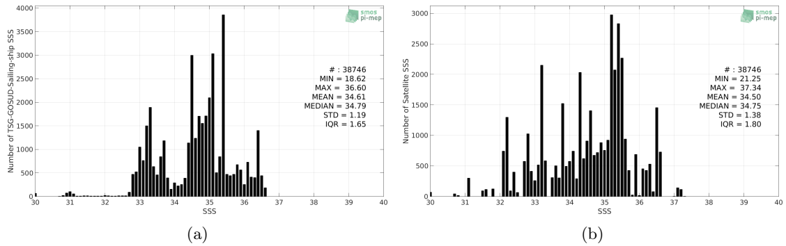
Figure 2: Histograms of SSS from TSG-GOSUD-Sailing-ship (a) and SMOS-L3-CATDS-CECOS-IFREMER-V2-1DAY-0.5DEG (b) considering all match-up pairs per bins of 0.1 over the Equatorial Ocean 10N-10S Pi-MEP region and for the full satellite product period.
