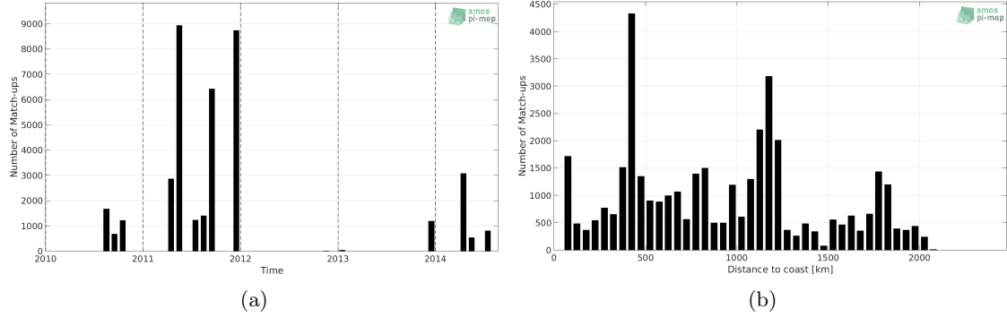
Figure 1: Number of match-ups between TSG-GOSUD-Sailing-ship and SMOS-L3-CATDS-CECOS-IFREMER-V2-1DAY-0.5DEG SSS as a function of time (a) and as function of the distance to coast (b) over the Equatorial Ocean 10N-10S Pi-MEP region and for the full satellite product period.
