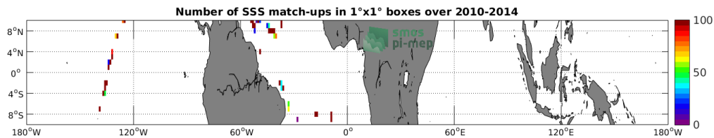
Figure 4: Number of SSS match-ups between TSG-GOSUD-Sailing-ship SSS and the SMOS-L3-CATDS-CECOS-IFREMER-V2-1DAY-0.5DEG SSS product for the Equatorial Ocean 10N-10S Pi-MEP region over 1^\circ \times 1^\circ boxes and for the full satellite product period.
