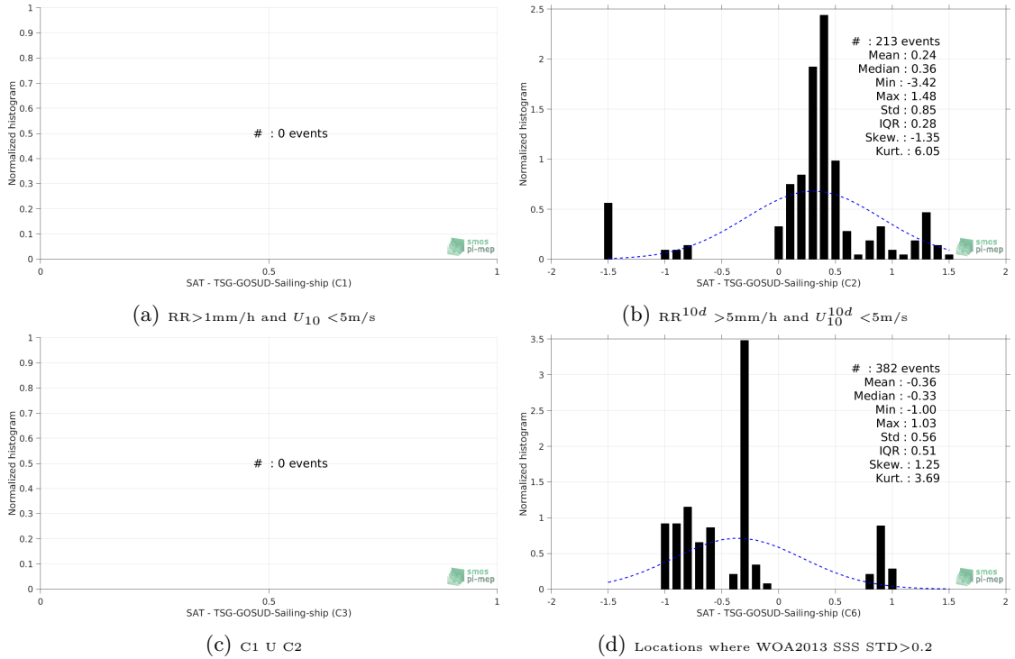
Figure 13: Normalized histogram of \Delta SSS (SMOS-L3-CATDS-CECOS-IFREMER-V2-1DAY-0.5DEG - TSG-GOSUD-Sailing-ship) for 6 different subdatasets corresponding to: RR > 1\text{mm/h} and U_{10} < 5\text{m/s} (a), RR^{10d} > 5\text{mm/h} and U_{10}^{10d} < 5\text{m/s} (b), C1 U C2 (c), Locations where WOA2013 SSS STD > 0.2 (d).
