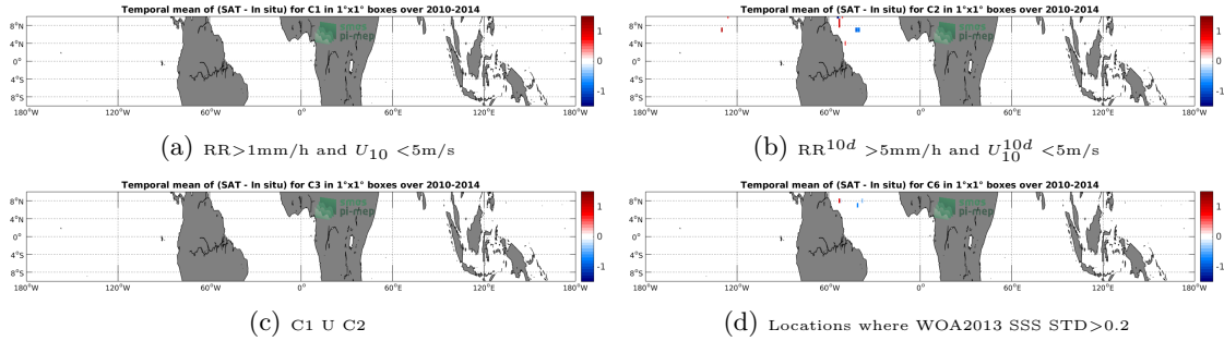
Figure 12: Temporal mean gridded over spatial boxes of size 1^\circ \times 1^\circ of \Delta SSS (SMOS-L3-CATDS-CECOS-IFREMER-V2-1DAY-0.5DEG - TSG-GOSUD-Sailing-ship) for 4 different subdatasets corresponding to: RR > 1\text{mm/h} and U_{10} < 5\text{m/s} (a), RR^{10d} > 5\text{mm/h} and U_{10}^{10d} < 5\text{m/s} (b), C1 U C2 (c), Locations where WOA2013 SSS STD > 0.2 (d).
