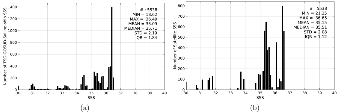
Figure 2: Histograms of SSS from TSG-GOSUD-Sailing-ship (a) and SMOS-L3-CATDS-CECOS-IFREMER-V2-1DAY-0.5deg (b) considering all match-up pairs per bins of 0.1 over the Equatorial Ocean 10N-10S Pi-MEP region and for the full satellite product period.
