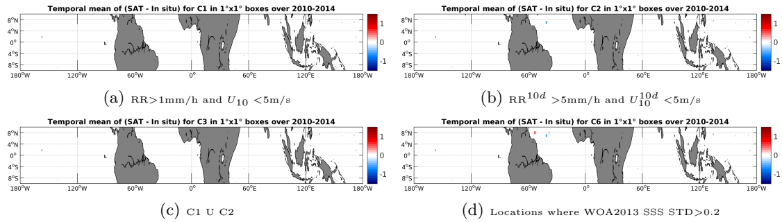
Figure 12: Temporal mean gridded over spatial boxes of size 1^\circ \times 1^\circ of \Delta SSS (SMOS-L3-CATDS-CECOS-IFREMER-V2-1DAY-0.5deg - TSG-GOSUD-Sailing-ship) for 4 different subdatasets corresponding to: RR > 1\text{mm/h} and U_{10} < 5\text{m/s} (a), RR^{10d} > 5\text{mm/h} and U_{10}^{10d} < 5\text{m/s} (b), C1 U C2 (c), Locations where WOA2013 SSS STD > 0.2 (d).
