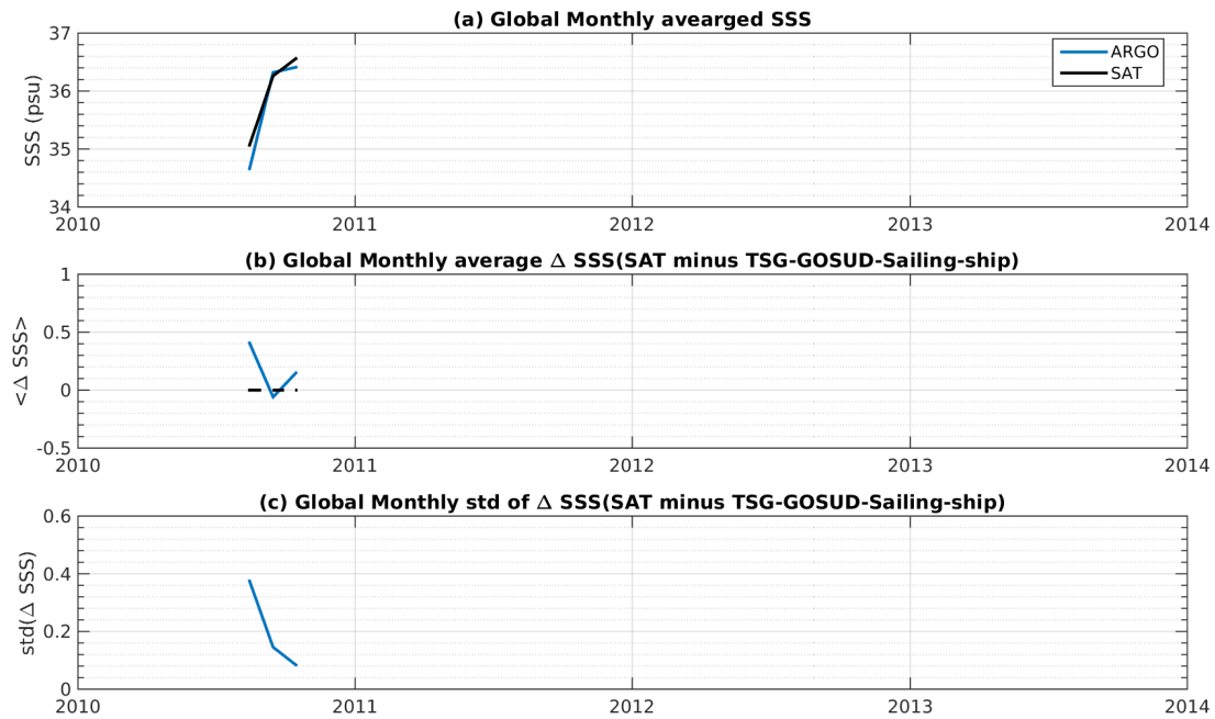
Figure 7: Time series of the monthly averaged mean SSS (top), mean \Delta SSS (Satellite - TSG-GOSUD-Sailing-ship) and STD of \Delta SSS (Satellite - TSG-GOSUD-Sailing-ship) over the Equatorial Ocean 10N-10S Pi-MEP region considering all match-ups collected by the Pi-MEP platform.
