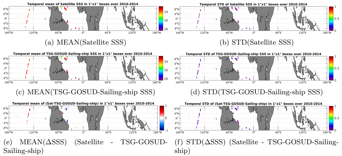
Figure 6: Temporal mean (left) and STD (right) of SSS from SMOS-L3-CATDS-CECOS-IFREMER-V2-1DAY-0.5deg (top), TSG-GOSUD-Sailing-ship (middle), and of \Delta SSS (Satellite - TSG-GOSUD-Sailing-ship). Only match-up pairs are used to generate these maps.
