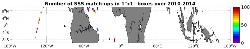
Figure 4: Number of SSS match-ups between TSG-GOSUD-Sailing-ship SSS and the SMOS-L3-CATDS-CECOS-IFREMER-V2-1DAY-0.5deg SSS product for the Equatorial Ocean 10N-10S Pi-MEP region over 1°x1° boxes and for the full satellite product period.
