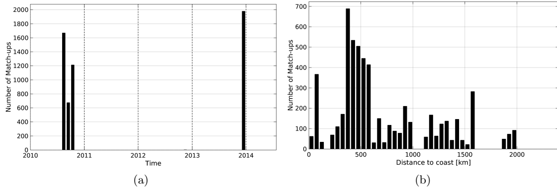
Figure 1: Number of match-ups between TSG-GOSUD-Sailing-ship and SMOS-L3-CATDS-CECOS-IFREMER-V2-1DAY-0.5deg SSS as a function of time (a) and as function of the distance to coast (b) over the Equatorial Ocean 10N-10S Pi-MEP region and for the full satellite product period.
