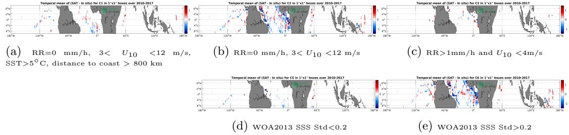
Figure 12: Temporal mean gridded over spatial boxes of size 1^{\circ}\times 1^{\circ} of \Delta SSS (SMOS SSS L3 v2 - Daily - 0.5 Deg (CATDS-CECOS-IFREMER) - TSG (GOSUD-Research-vessel)) for 5 different subdatasets corresponding to:RR=0 mm/h, 3 < U_{10} < 12 m/s, SST >5^{\circ}\text{C} , distance to coast > 800 km (a), RR=0 mm/h, 3 < U_{10} < 12 m/s (b), RR >1 mm/h and U_{10} < 4 m/s (c), WOA2013 SSS Std <0.2 (d), WOA2013 SSS Std >0.2 (e).
