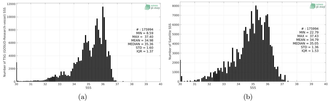
Figure 2: Histograms of SSS from TSG (GOSUD-Research-vessel) (a) and SMOS SSS L3 v2 - Daily - 0.5 Deg (CATDS-CECOS-IFREMER) (b) considering all match-up pairs per bins of 0.1 over the Equatorial Ocean 10N-10S Pi-MEP region and for the full satellite product period.
