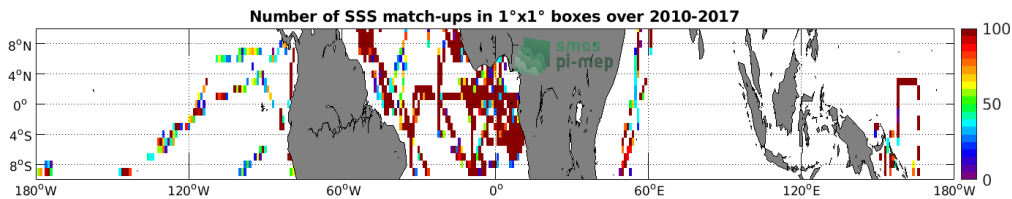
Figure 4: Number of SSS match-ups between TSG (GOSUD-Research-vessel) SSS and the SMOS SSS L3 v2 - Daily - 0.5 Deg (CATDS-CECOS-IFREMER) SSS product for the Equatorial Ocean 10N-10S Pi-MEP region over 1^\circ \times 1^\circ boxes and for the full satellite product period.
