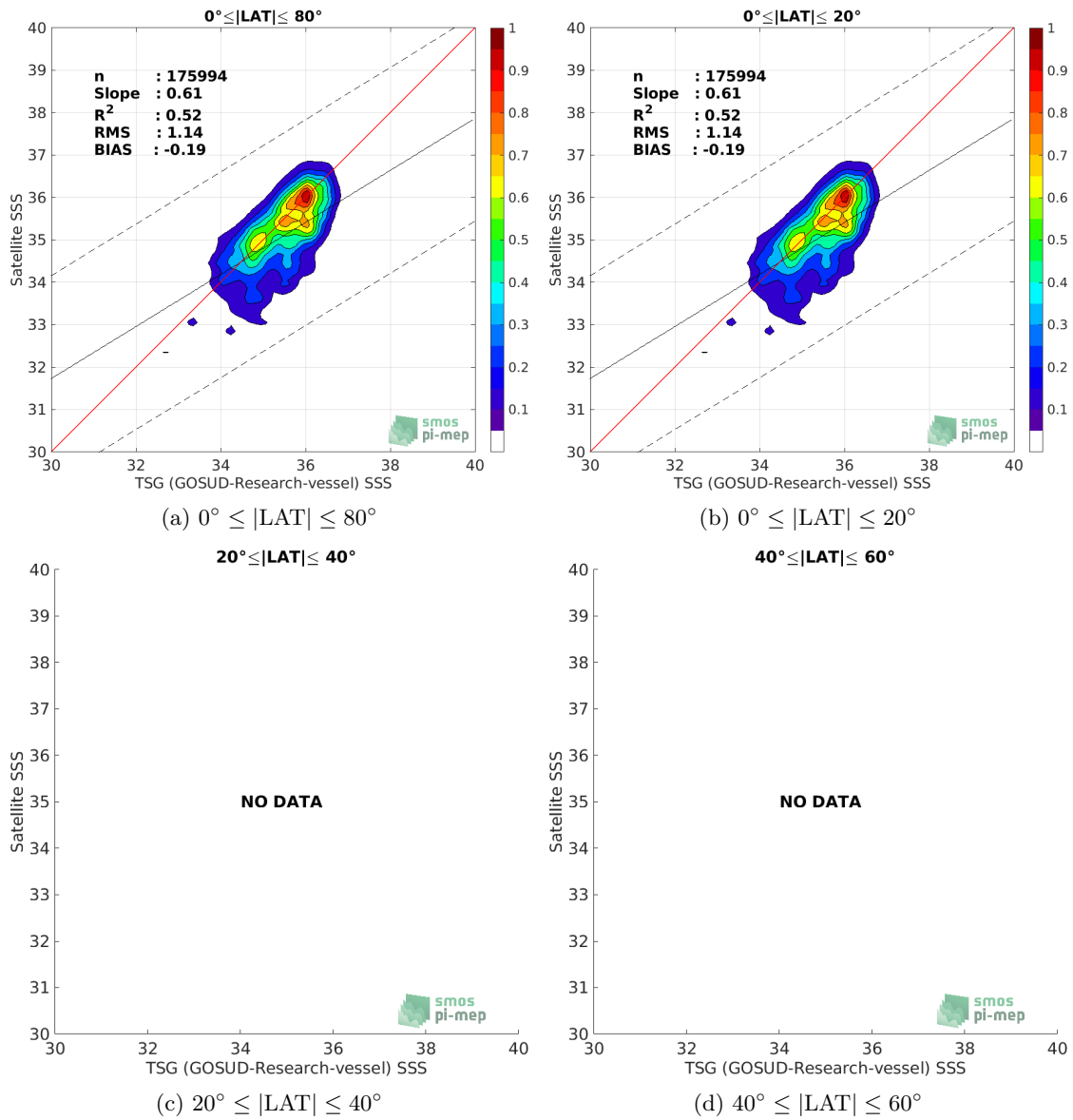
Figure 9: Contour maps of the concentration of SMOS SSS L3 v2 - Daily - 0.5 Deg (CATDS-CECOS-IFREMER) SSS (y-axis) versus TSG (GOSUD-Research-vessel) SSS (x-axis) at match-up pairs for different latitude bands. For each plot, the red line shows x=y . The black thin and dashed lines indicate a linear fit through the data cloud and the \pm 95\% confidence levels, respectively. The number match-up pairs n , the slope and R^2 coefficient of the linear fit, the root mean square (RMS) and the mean bias between satellite and in situ data are indicated for each latitude band in each plots.
