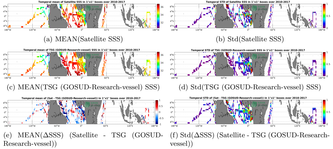
Figure 6: Temporal mean (left) and Std (right) of SSS from SMOS SSS L3 v2 - Daily - 0.5 Deg (CATDS-CECOS-IFREMER) (top), TSG (GOSUD-Research-vessel) (middle), and of \Delta SSS (Satellite - TSG (GOSUD-Research-vessel)). Only match-up pairs are used to generate these maps.
