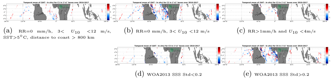
Figure 12: Temporal mean gridded over spatial boxes of size 1^{\circ}\times 1^{\circ} of \Delta SSS (SMOS L3 v2 - Daily - 0.5 Deg (CATDS-CECOS-IFREMER) - TSG-GOSUD-Research-vessel) for 5 different subdatasets corresponding to:RR=0 mm/h, 3 < U_{10} < 12 m/s, SST >5^{\circ}\text{C} , distance to coast > 800 km (a), RR=0 mm/h, 3 < U_{10} < 12 m/s (b), RR >1 mm/h and U_{10} < 4 m/s (c), WOA2013 SSS Std <0.2 (d), WOA2013 SSS Std >0.2 (e).
