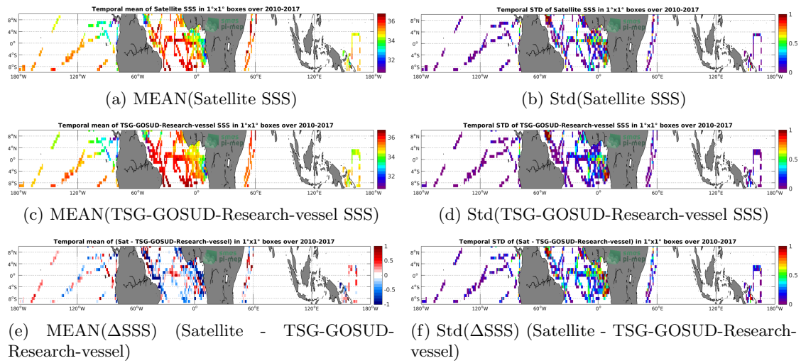
Figure 6: Temporal mean (left) and Std (right) of SSS from SMOS L3 v2 - Daily - 0.5 Deg (CATDS-CECOS-IFREMER) (top), TSG-GOSUD-Research-vessel (middle), and of \Delta SSS (Satellite - TSG-GOSUD-Research-vessel). Only match-up pairs are used to generate these maps.
